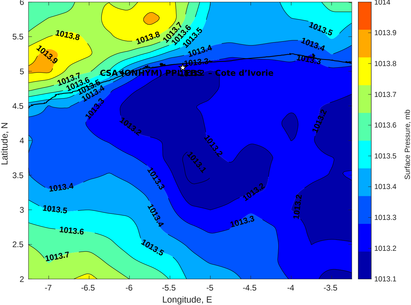
Surface Pressure (mb) for CSA (ONHYM) PPL EBS - Cote d'Ivoire at 15-Oct-2025 00:00:00
