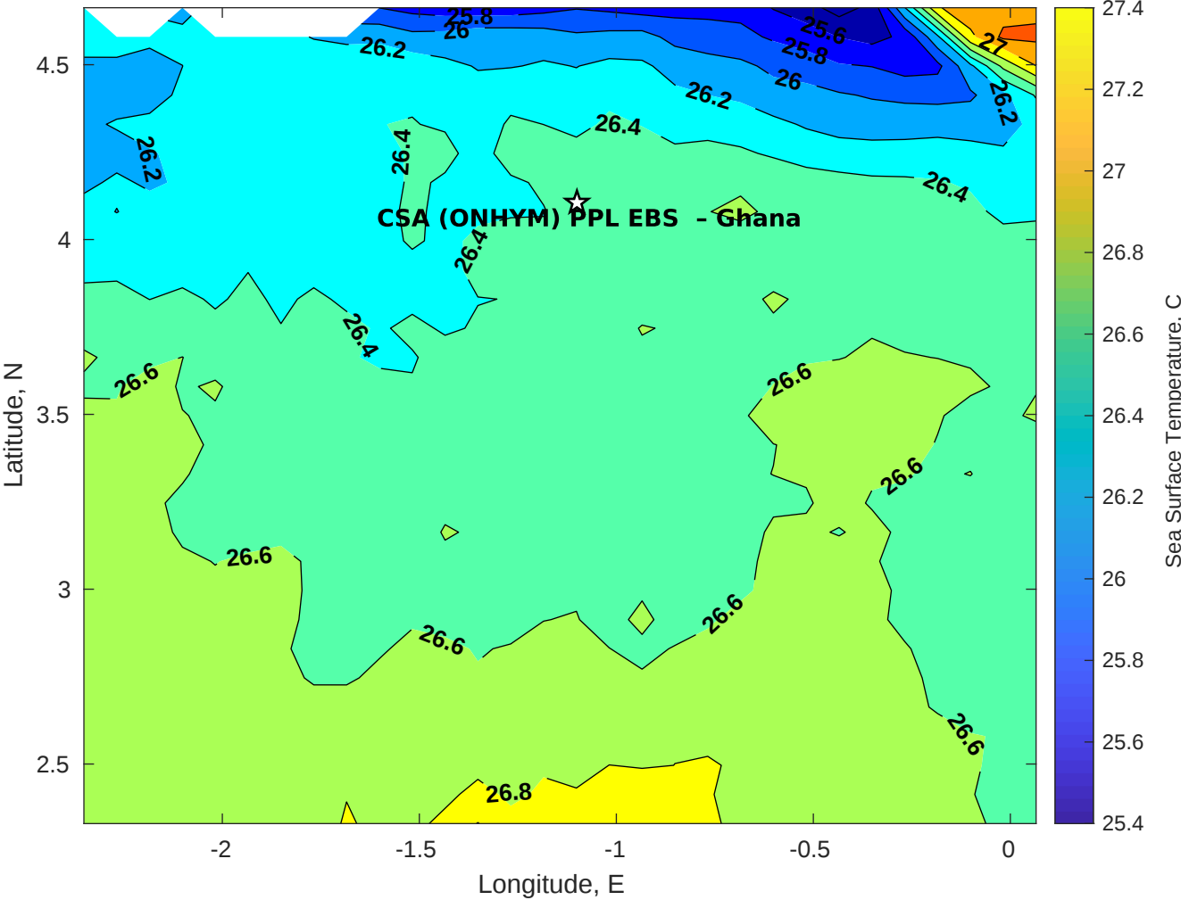
SST for CSA (ONHYM) PPL EBS - Ghana at 12-Oct-2025 00:00:00
