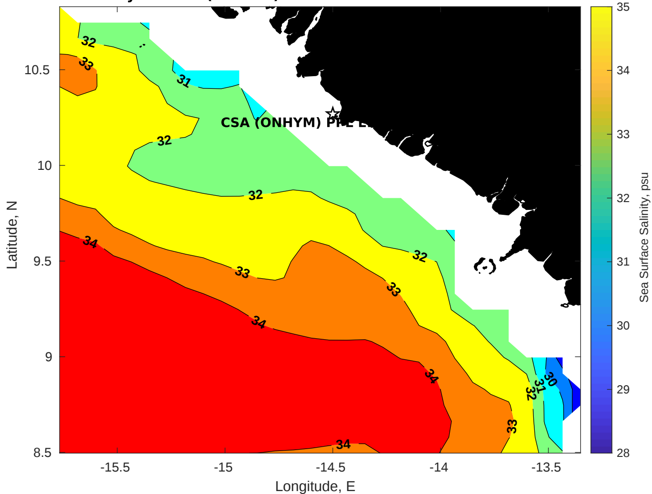
Surface Salinity for CSA (ONHYM) PPL EBS - Guinea at 12-Oct-2025 00:00:00
