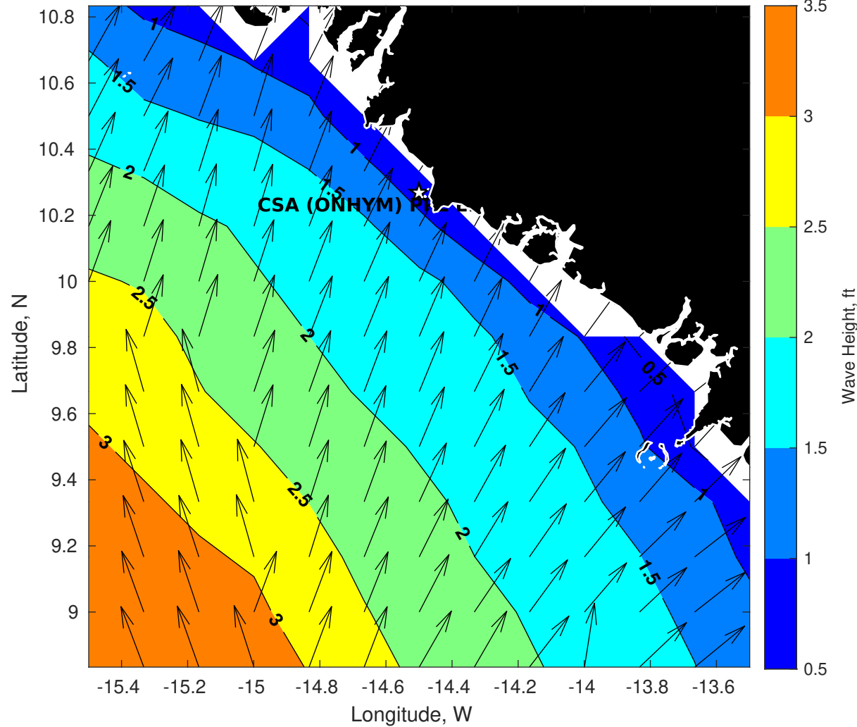
Wave Height (ft) for CSA (ONHYM) PPL EBS - Guinea at 13-Oct-2025 09:00:00
