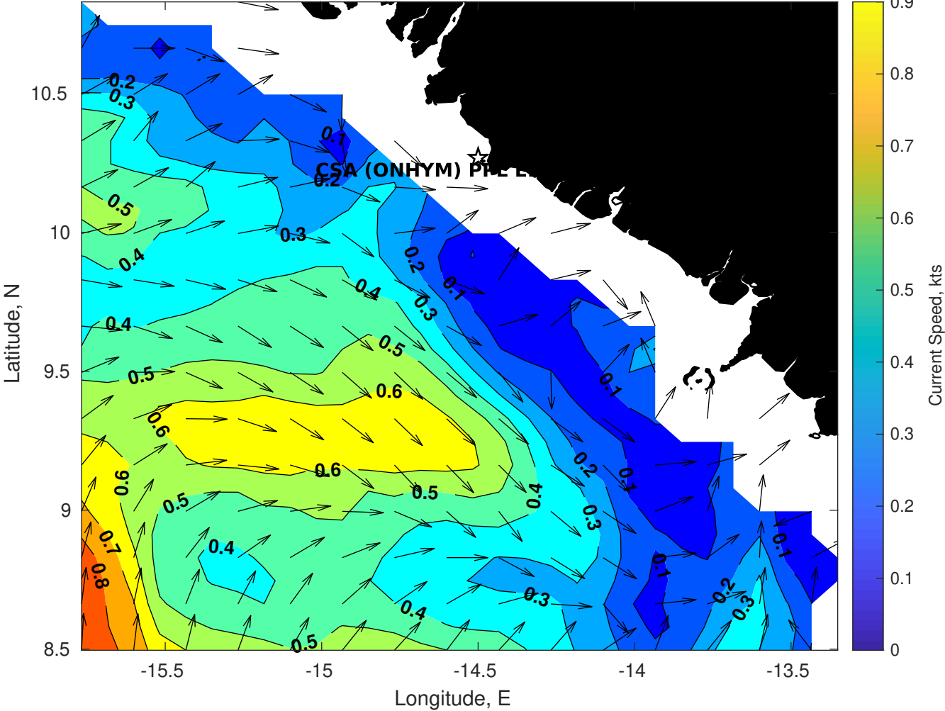
Surface Currents for CSA (ONHYM) PPL EBS - Guinea at 12-Oct-2025 00:00:00
