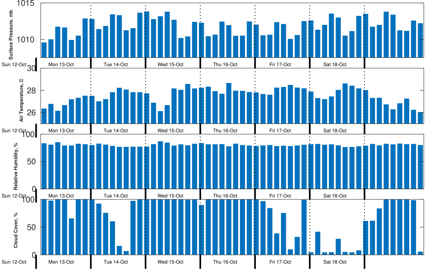
Met Forecast for CSA (ONHYM) PPL EBS - Guinea from 13-Oct-2025 00:00:00 to 20-Oct-2025 00:00:00
