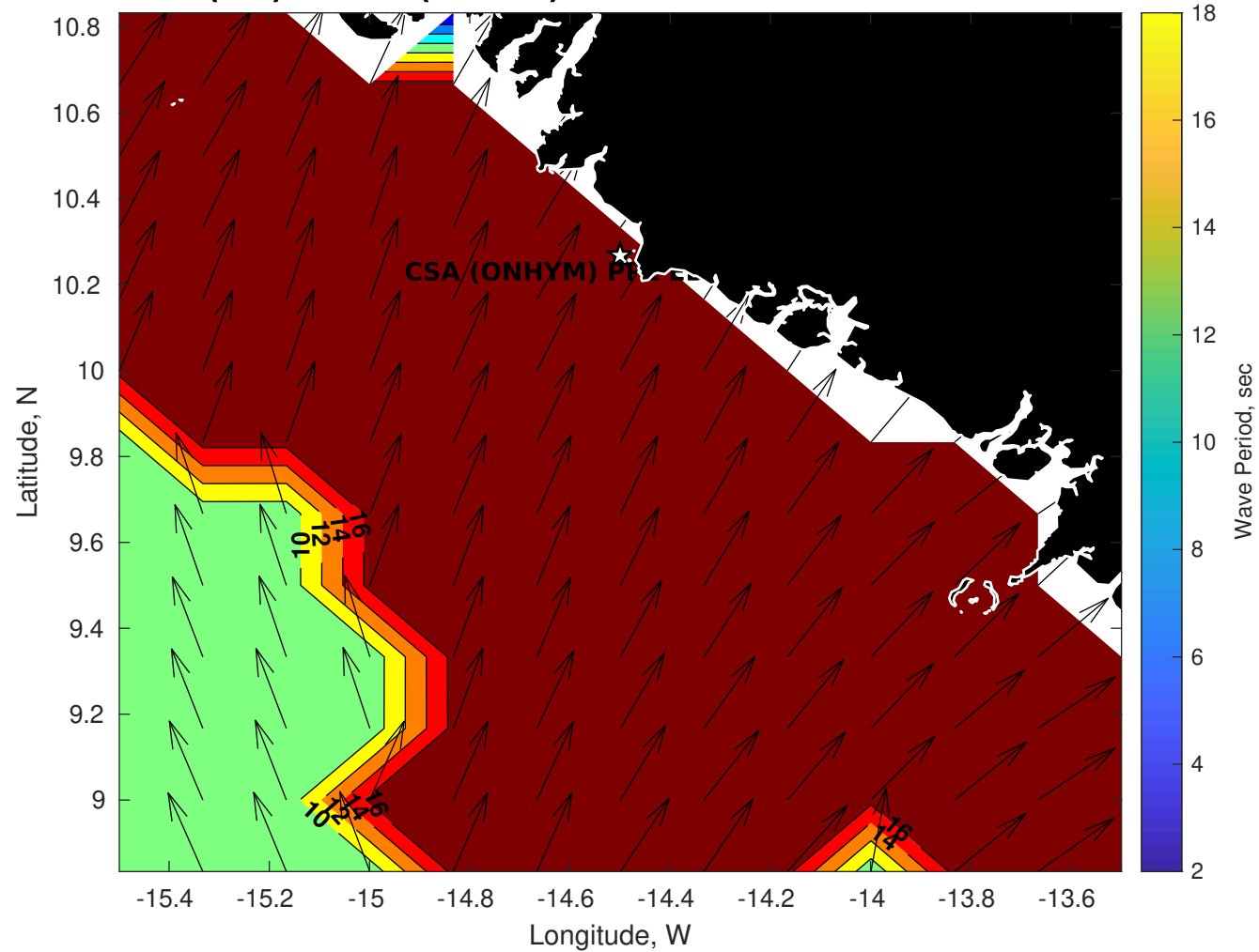
Wave Period (sec) for CSA (ONHYM) PPL EBS - Guinea at 13-Oct-2025 09:00:00
