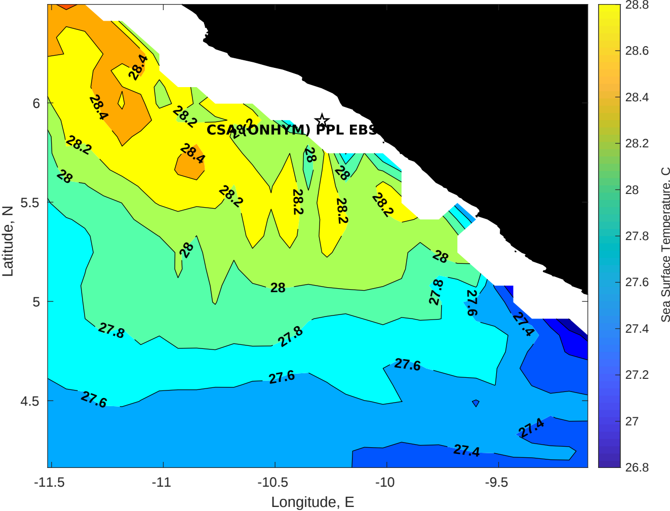
SST for CSA (ONHYM) PPL EBS - Liberia at 12-Oct-2025 00:00:00
