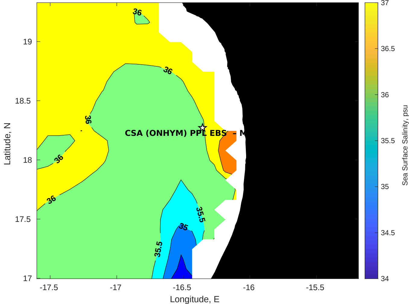
Surface Salinity for CSA (ONHYM) PPL EBS - Mauritania at 12-Oct-2025 00:00:00
