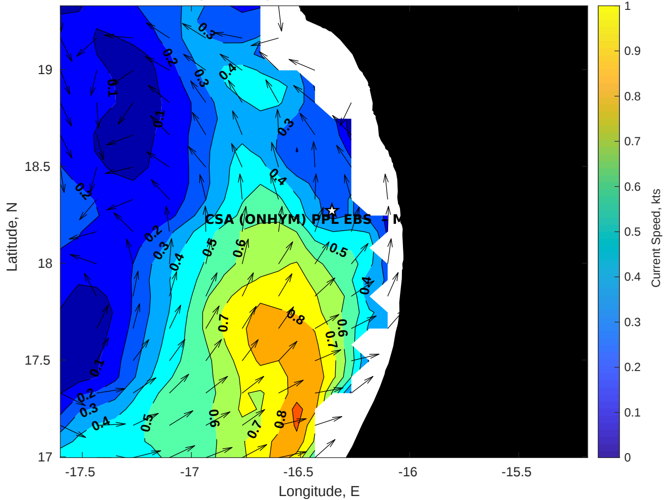
Surface Currents for CSA (ONHYM) PPL EBS - Mauritania at 12-Oct-2025 00:00:00
