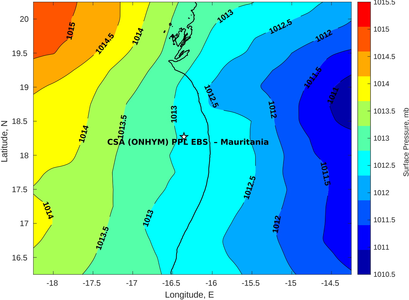
Surface Pressure (mb) for CSA (ONHYM) PPL EBS - Mauritania at 15-Oct-2025 00:00:00
