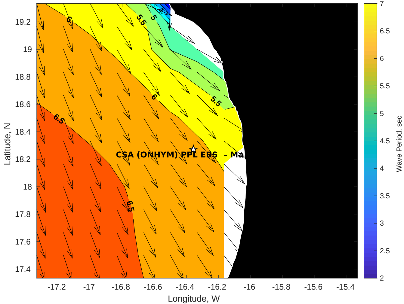
Wave Period (sec) for CSA (ONHYM) PPL EBS - Mauritania at 13-Oct-2025 09:00:00
