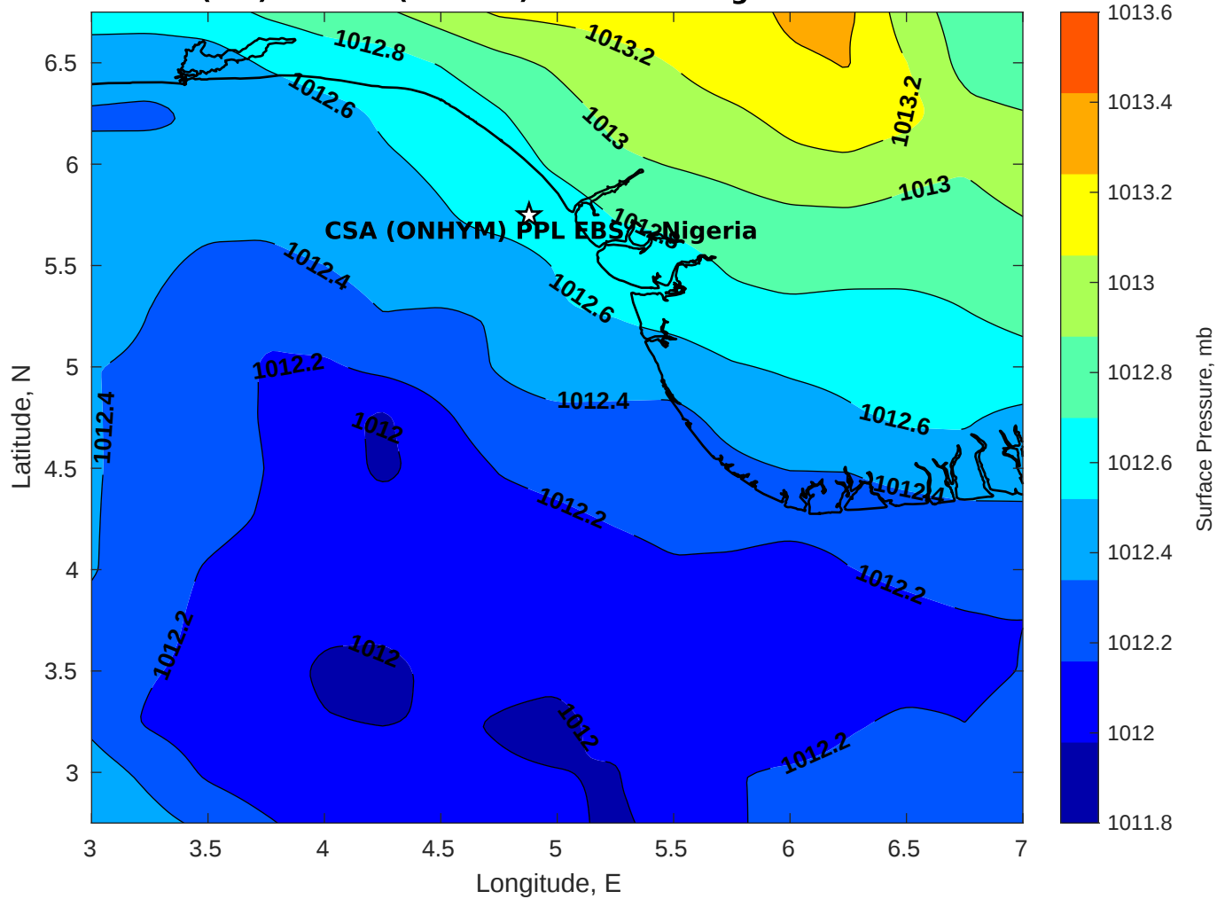
Surface Pressure (mb) for CSA (ONHYM) PPL EBS - Nigeria at 15-Oct-2025 00:00:00
