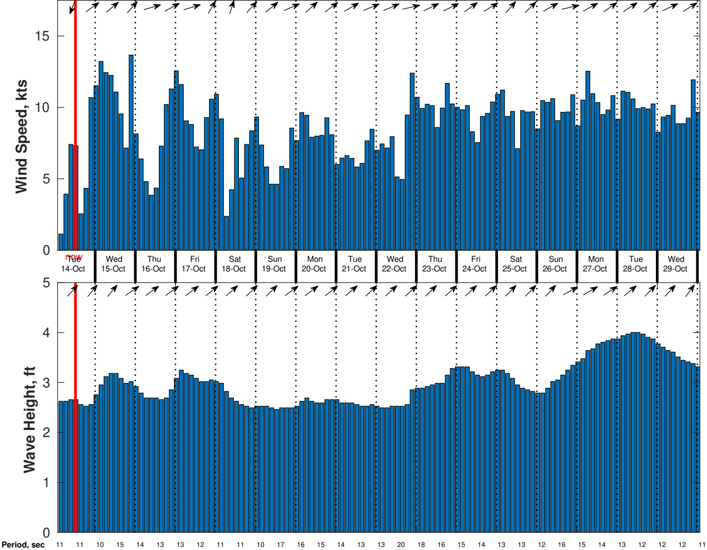
Wind & Wave Forecast for CSA (ONHYM) PPL EBS - Nigeria from 13-Oct-2025 02:00:00 to 29-Oct-2025 02:00:00
