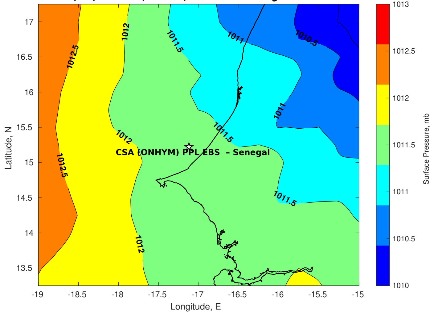
Surface Pressure (mb) for CSA (ONHYM) PPL EBS - Senegal at 14-Oct-2025 00:00:00
