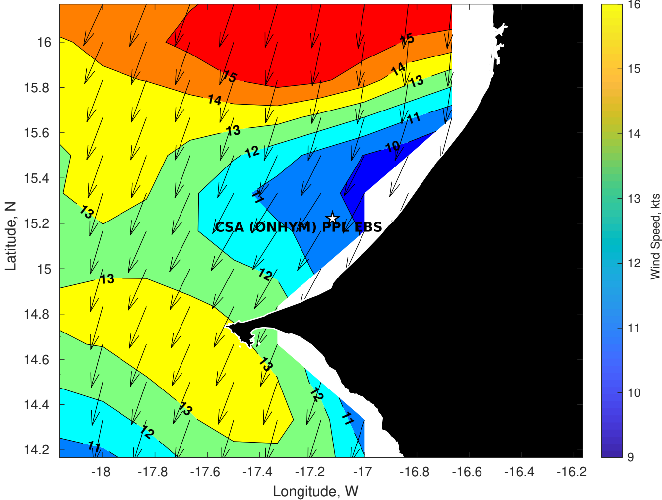
Winds (kts) for CSA (ONHYM) PPL EBS - Senegal at 13-Oct-2025 09:00:00
