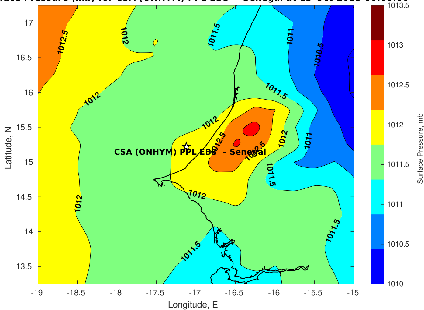
Surface Pressure (mb) for CSA (ONHYM) PPL EBS - Senegal at 13-Oct-2025 00:00:00
