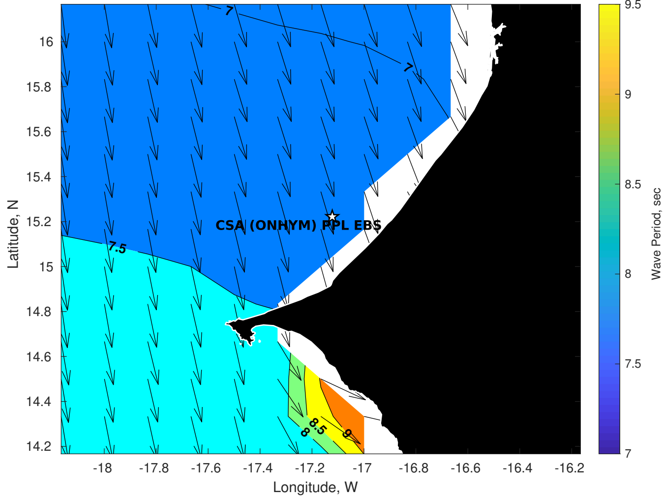
Wave Period (sec) for CSA (ONHYM) PPL EBS - Senegal at 13-Oct-2025 09:00:00
