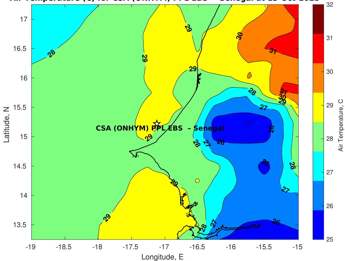
Air Temperature (C) for CSA (ONHYM) PPL EBS - Senegal at 13-Oct-2025
