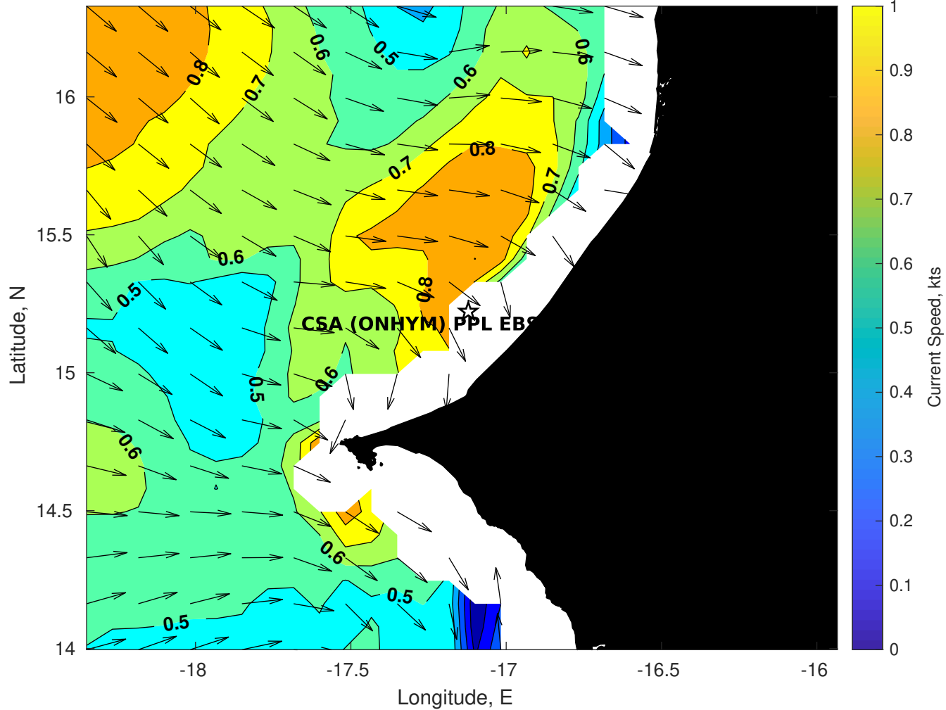
Surface Currents for CSA (ONHYM) PPL EBS - Senegal at 12-Oct-2025 00:00:00
