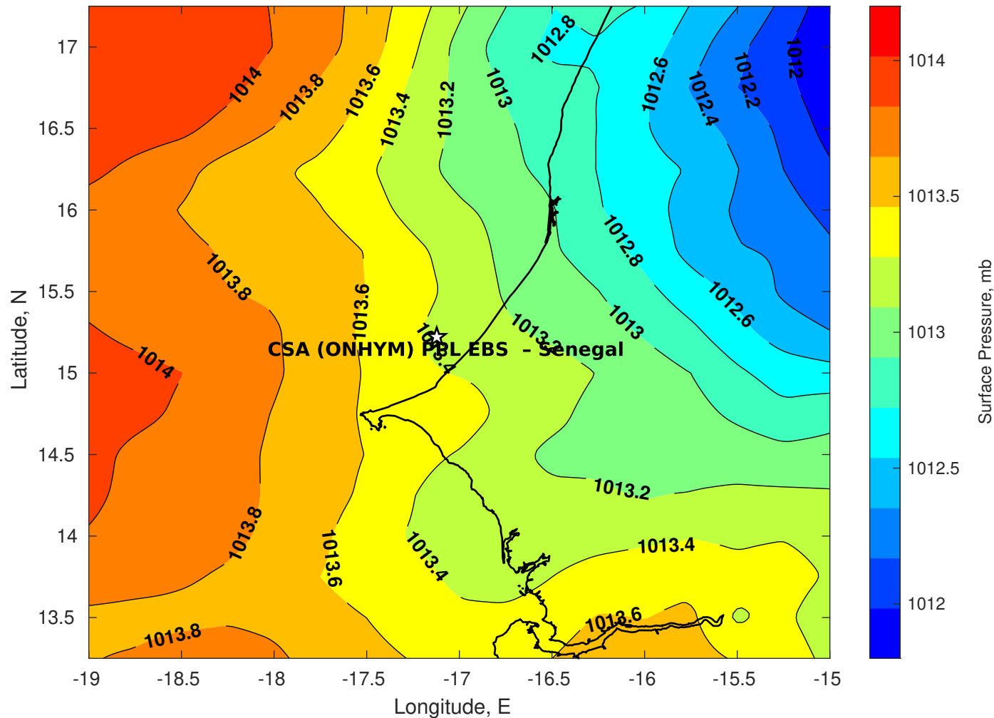
Surface Pressure (mb) for CSA (ONHYM) PPL EBS - Senegal at 15-Oct-2025 00:00:00
