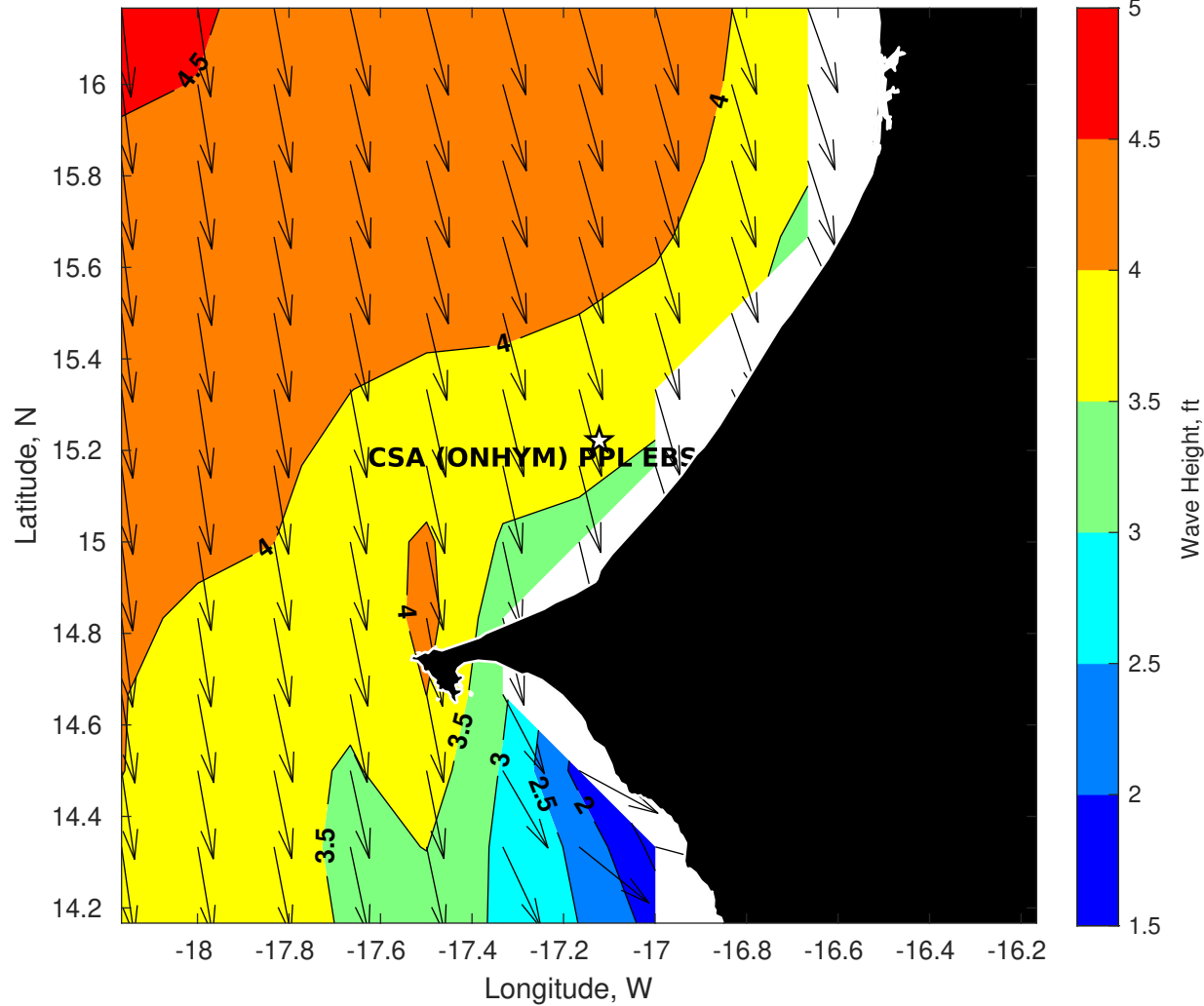
Wave Height (ft) for CSA (ONHYM) PPL EBS - Senegal at 13-Oct-2025 09:00:00
