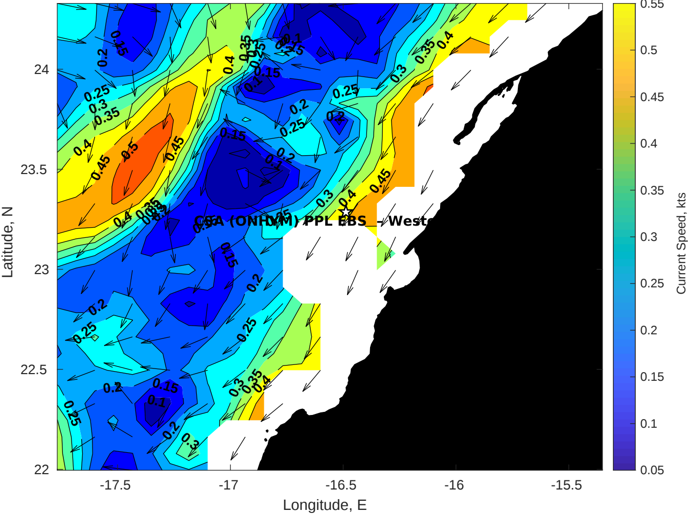
Surface Currents for CSA (ONHYM) PPL EBS - Western Sahara at 12-Oct-2025 00:00:00
