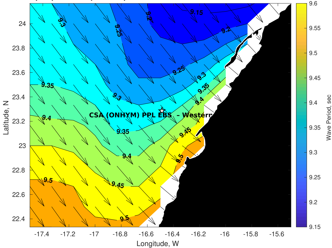
Wave Period (sec) for CSA (ONHYM) PPL EBS - Western Sahara at 13-Oct-2025 09:00:00
