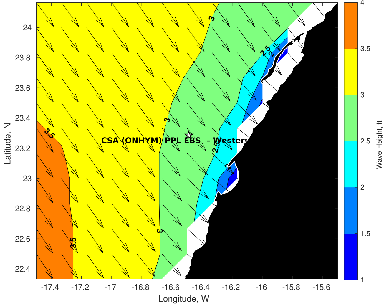
Wave Height (ft) for CSA (ONHYM) PPL EBS - Western Sahara at 13-Oct-2025 09:00:00
