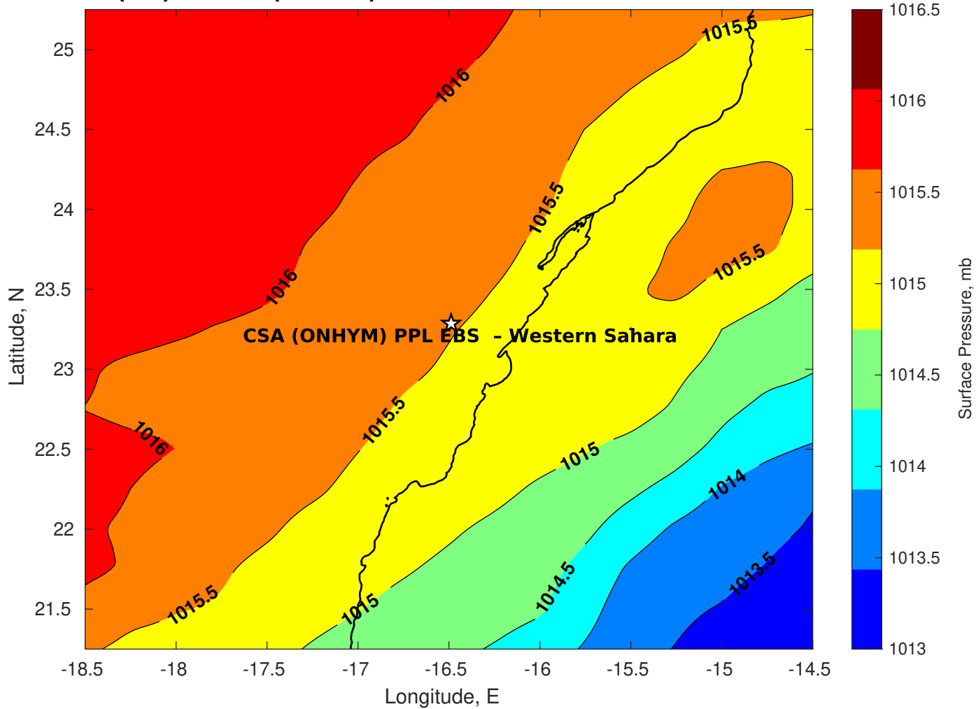
Surface Pressure (mb) for CSA (ONHYM) PPL EBS - Western Sahara at 15-Oct-2025 00:00:00
