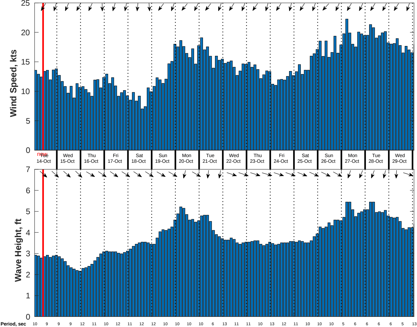
Wind & Wave Forecast for CSA (ONHYM) PPL EBS - Western Sahara from 13-Oct-2025 01:00:00 to 29-Oct-2025 01:00:00
