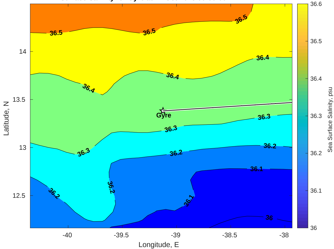
Surface Salinity for Gyre at 12-Oct-2025 00:00:00
