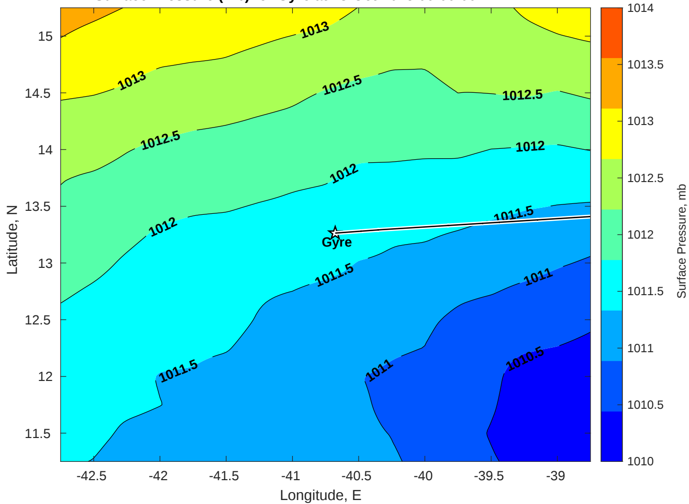
Surface Pressure (mb) for Gyre at 13-Oct-2025 00:00:00
