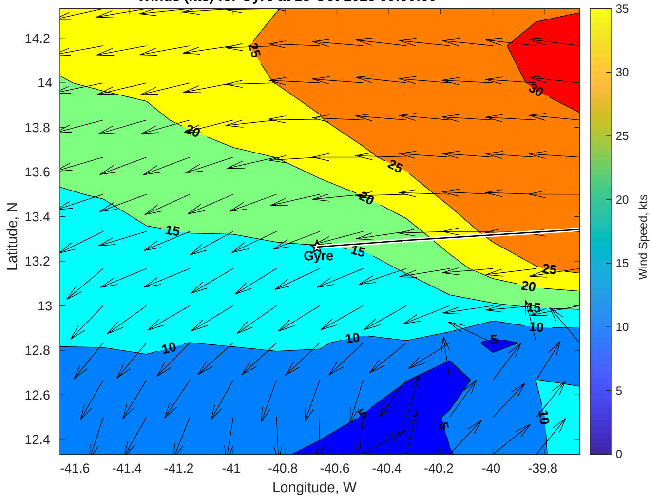
Winds (kts) for Gyre at 13-Oct-2025 09:00:00
