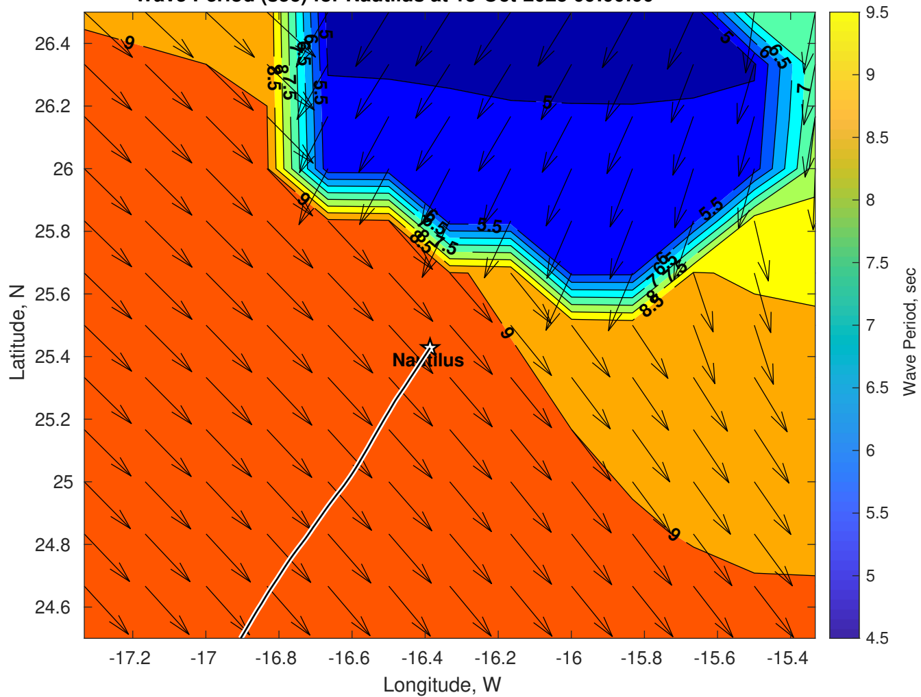
Wave Period (sec) for Nautilus at 13-Oct-2025 09:00:00
