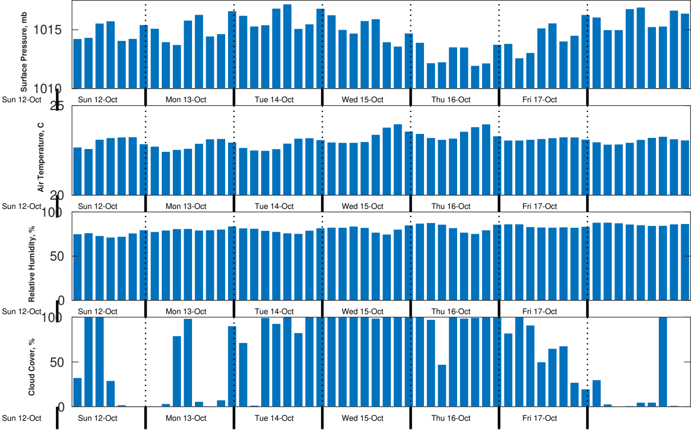
Met Forecast for Nautilus from 13-Oct-2025 00:00:00 to 20-Oct-2025 00:00:00
