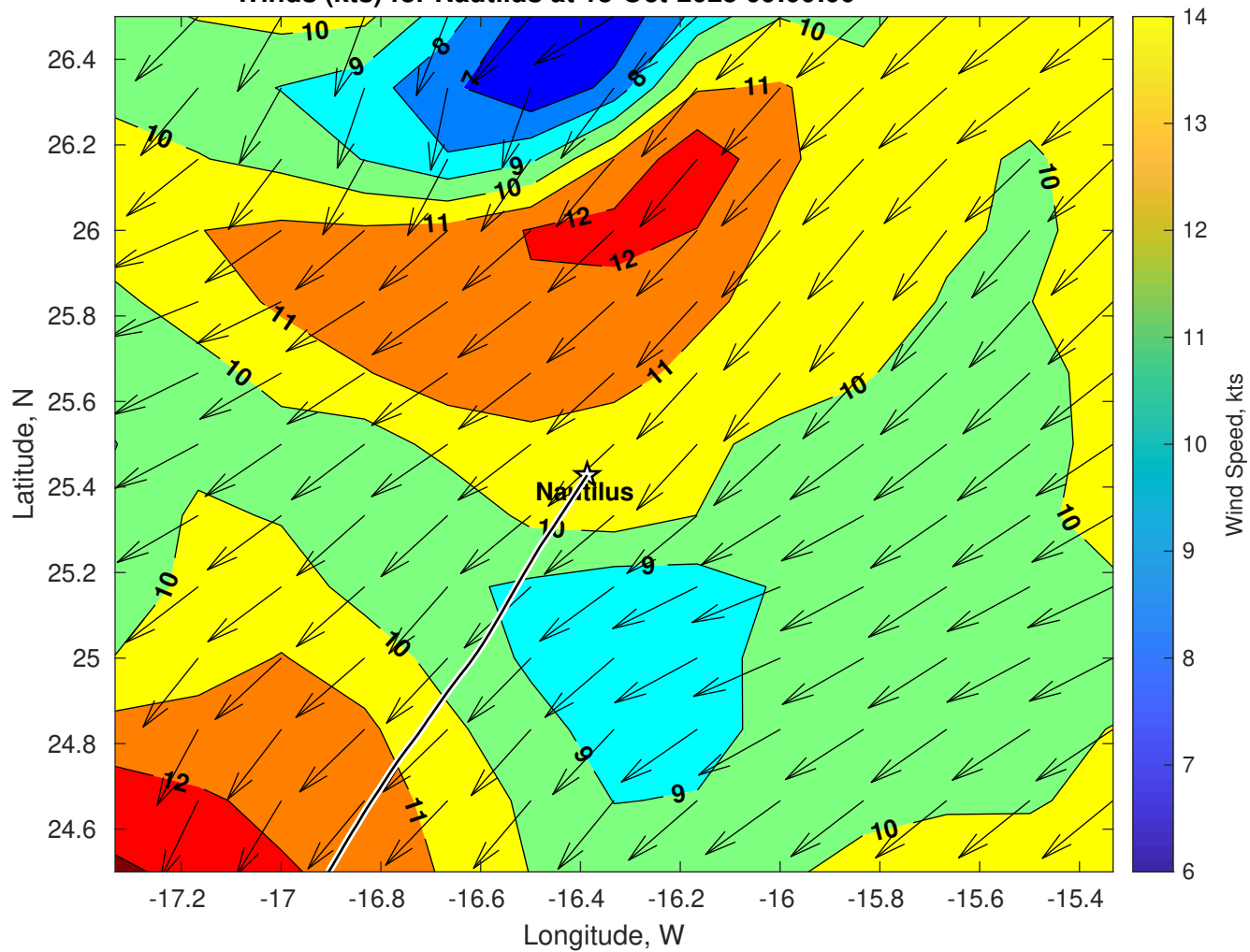
Winds (kts) for Nautilus at 13-Oct-2025 09:00:00
