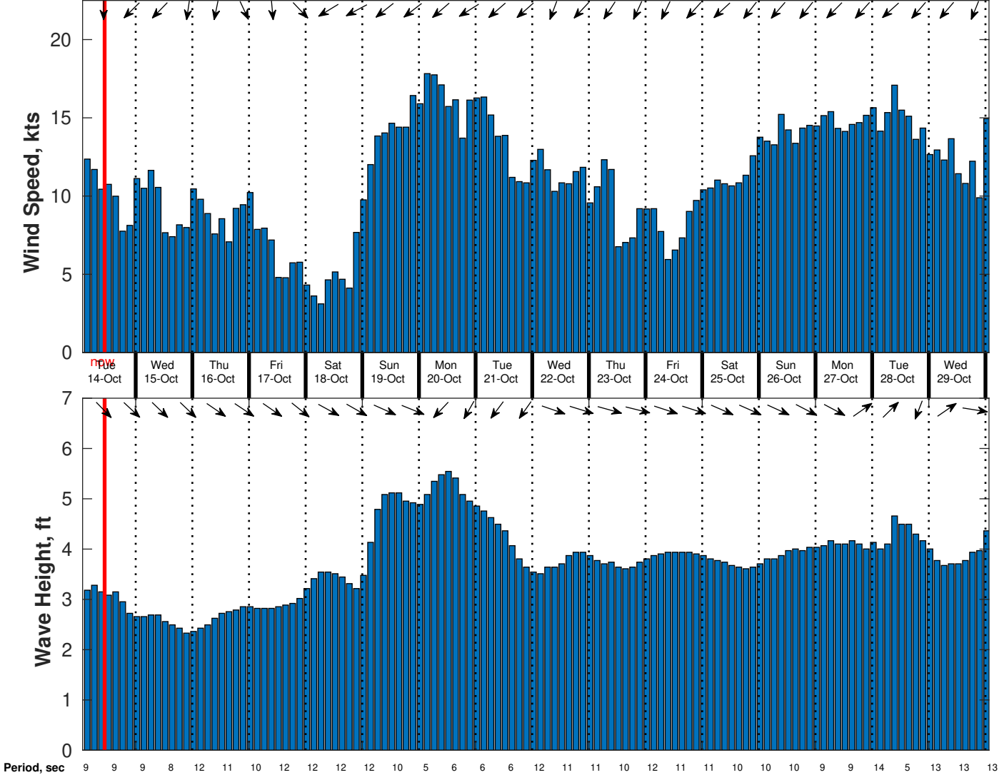
Wind & Wave Forecast for Nautilus from 13-Oct-2025 02:00:00 to 29-Oct-2025 02:00:00
