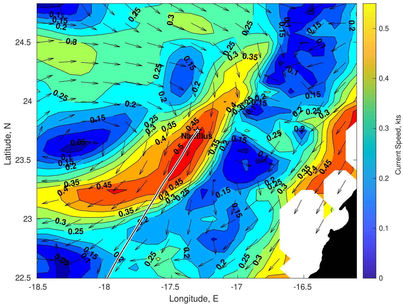
Surface Currents for Nautilus at 12-Oct-2025 00:00:00
