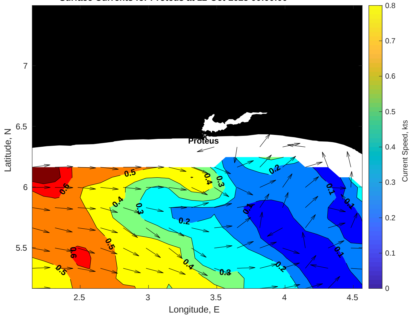
Surface Currents for Proteus at 12-Oct-2025 00:00:00
