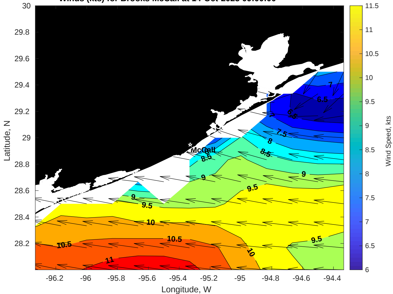
Winds (kts) for Brooks McCall at 14-Oct-2025 09:00:00
