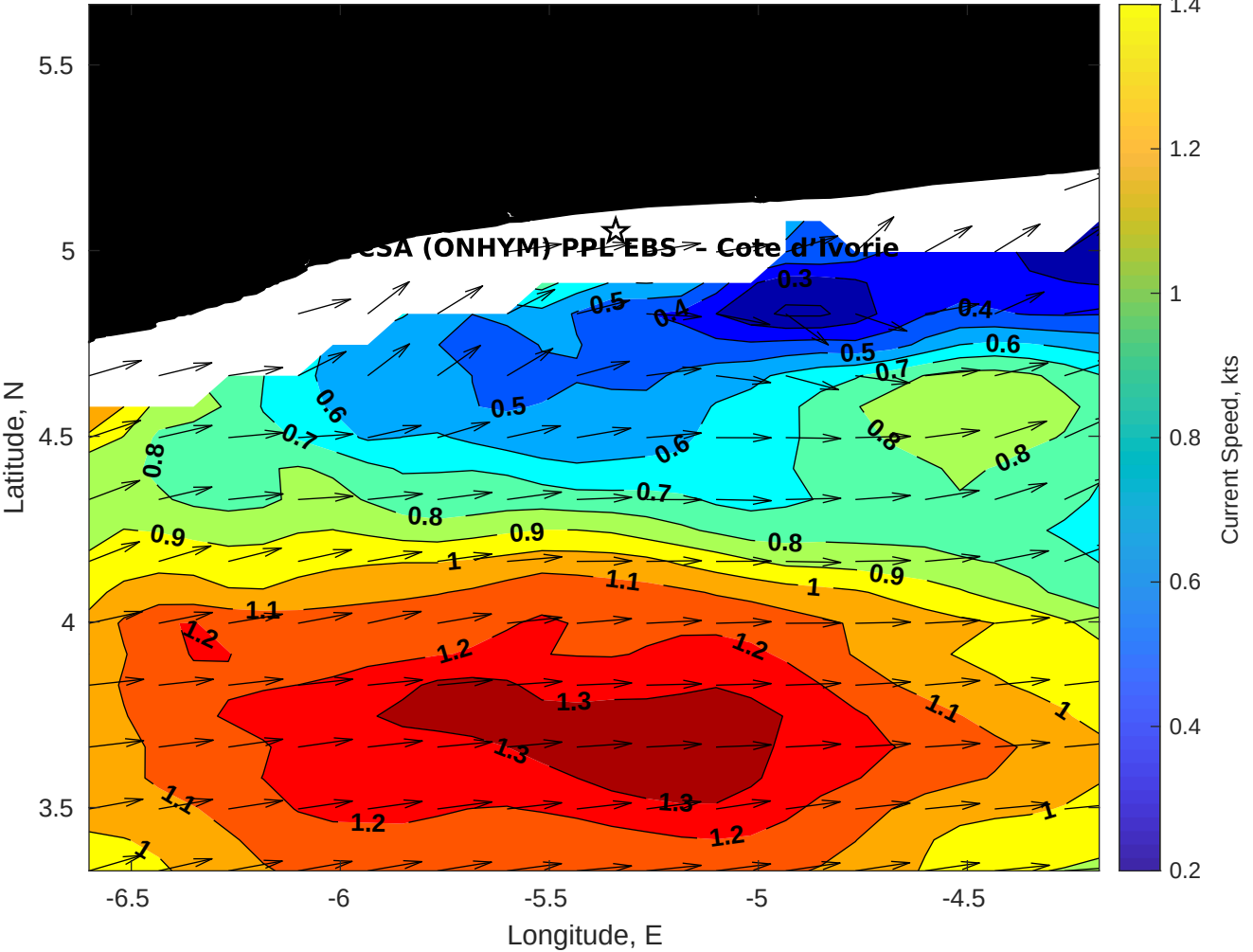
Surface Currents for CSA (ONHYM) PPL EBS - Cote d'Ivoire at 13-Oct-2025 00:00:00
