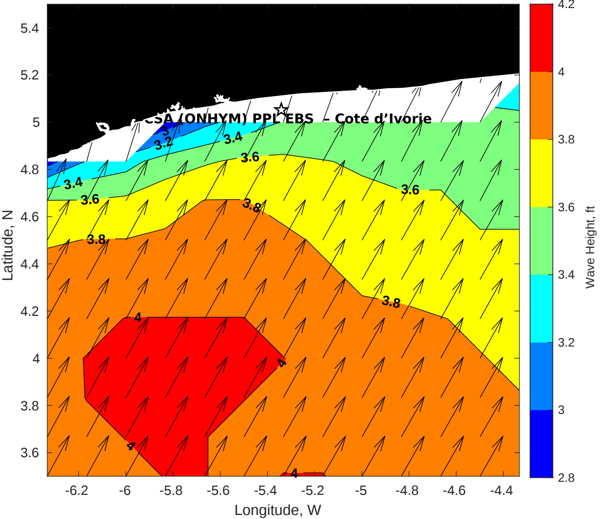
Wave Height (ft) for CSA (ONHYM) PPL EBS - Cote d'Ivoire at 14-Oct-2025 09:00:00
