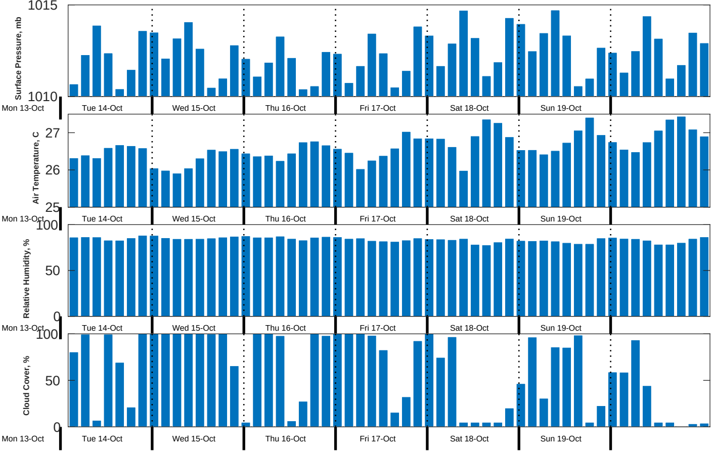
Met Forecast for CSA (ONHYM) PPL EBS - Cote d'Ivoire from 14-Oct-2025 00:00:00 to 21-Oct-2025 00:00:00
