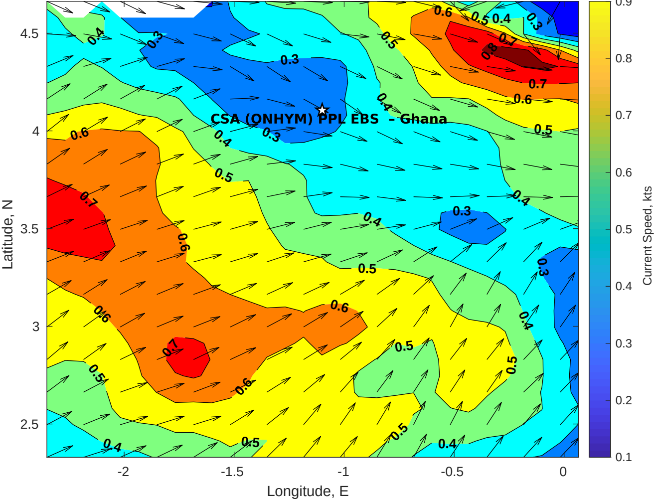
Surface Currents for CSA (ONHYM) PPL EBS - Ghana at 13-Oct-2025 00:00:00
