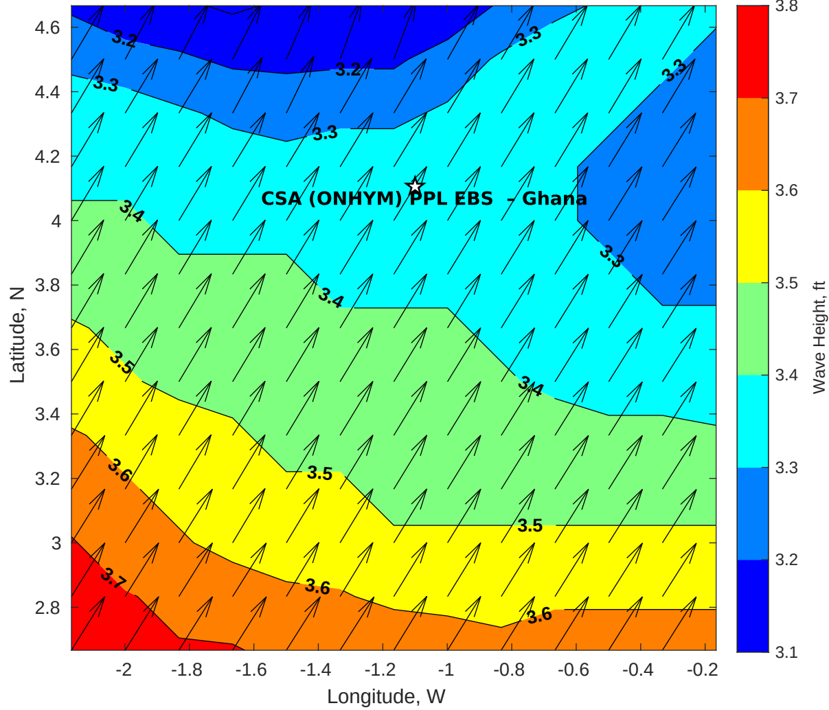
Wave Height (ft) for CSA (ONHYM) PPL EBS - Ghana at 14-Oct-2025 09:00:00
