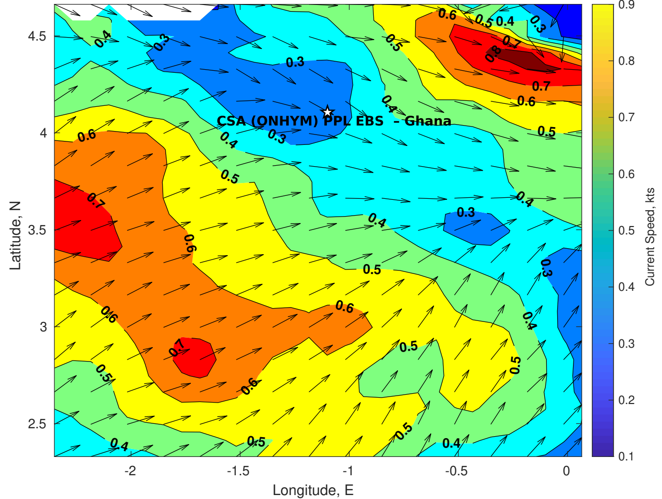
Surface Currents for CSA (ONHYM) PPL EBS - Ghana at 13-Oct-2025 00:00:00
