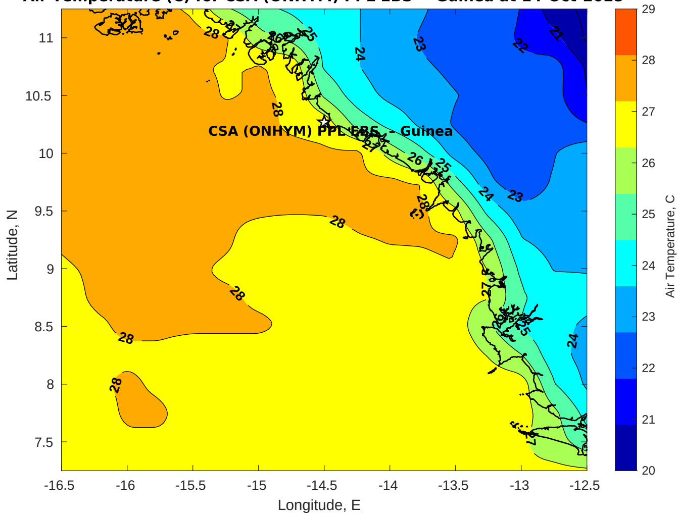
Air Temperature (C) for CSA (ONHYM) PPL EBS - Guinea at 14-Oct-2025
