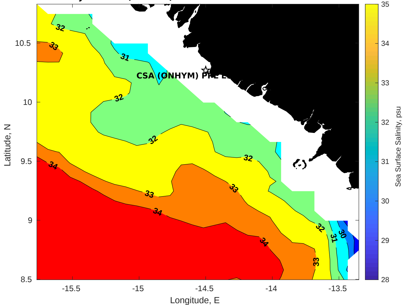
Surface Salinity for CSA (ONHYM) PPL EBS - Guinea at 13-Oct-2025 00:00:00
