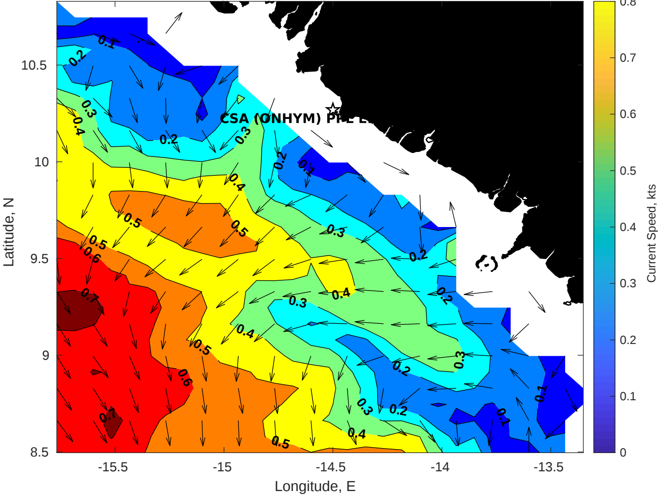
Surface Currents for CSA (ONHYM) PPL EBS - Guinea at 13-Oct-2025 00:00:00
