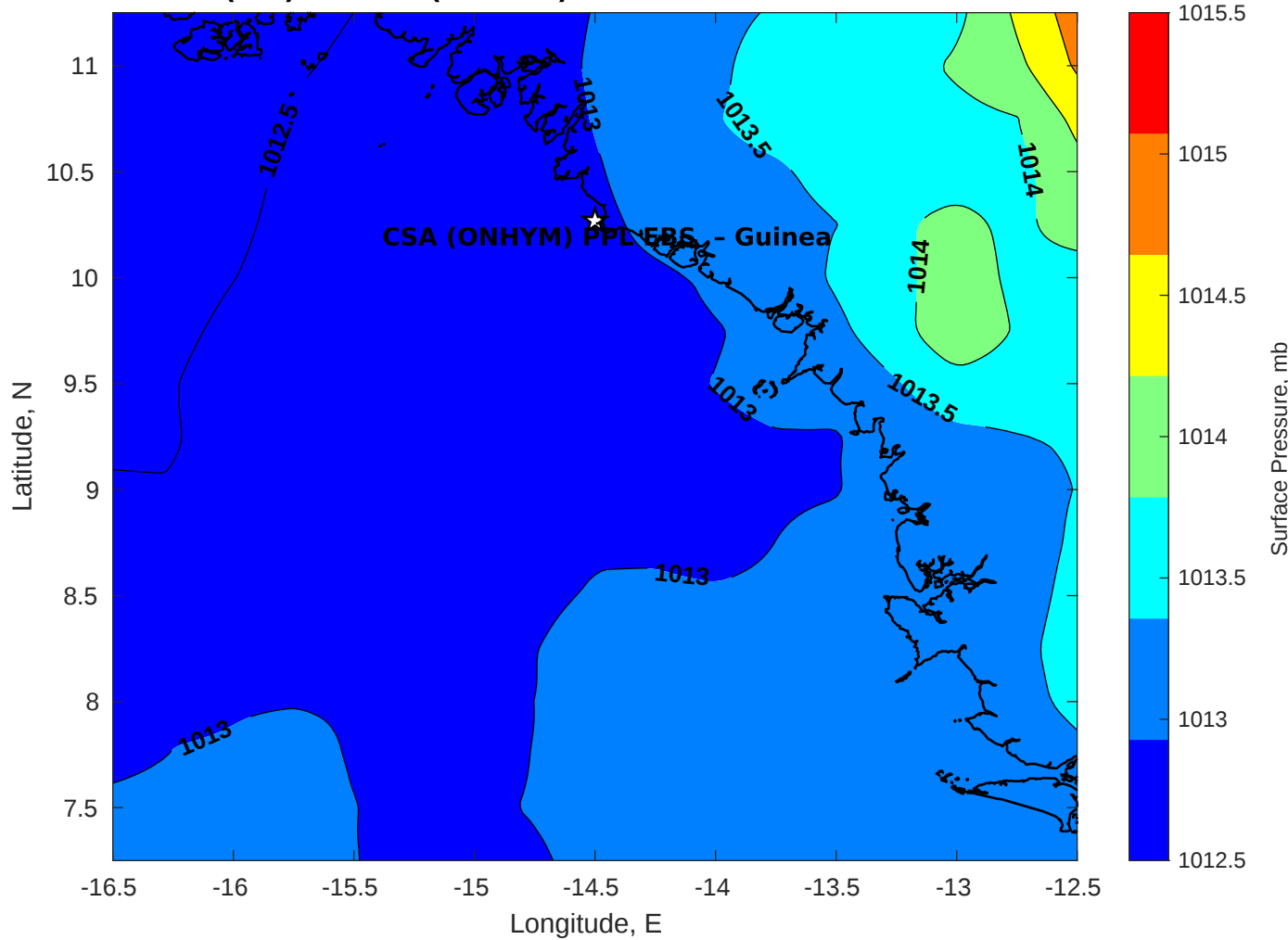
Surface Pressure (mb) for CSA (ONHYM) PPL EBS - Guinea at 03-Oct-2025 00:00:00
