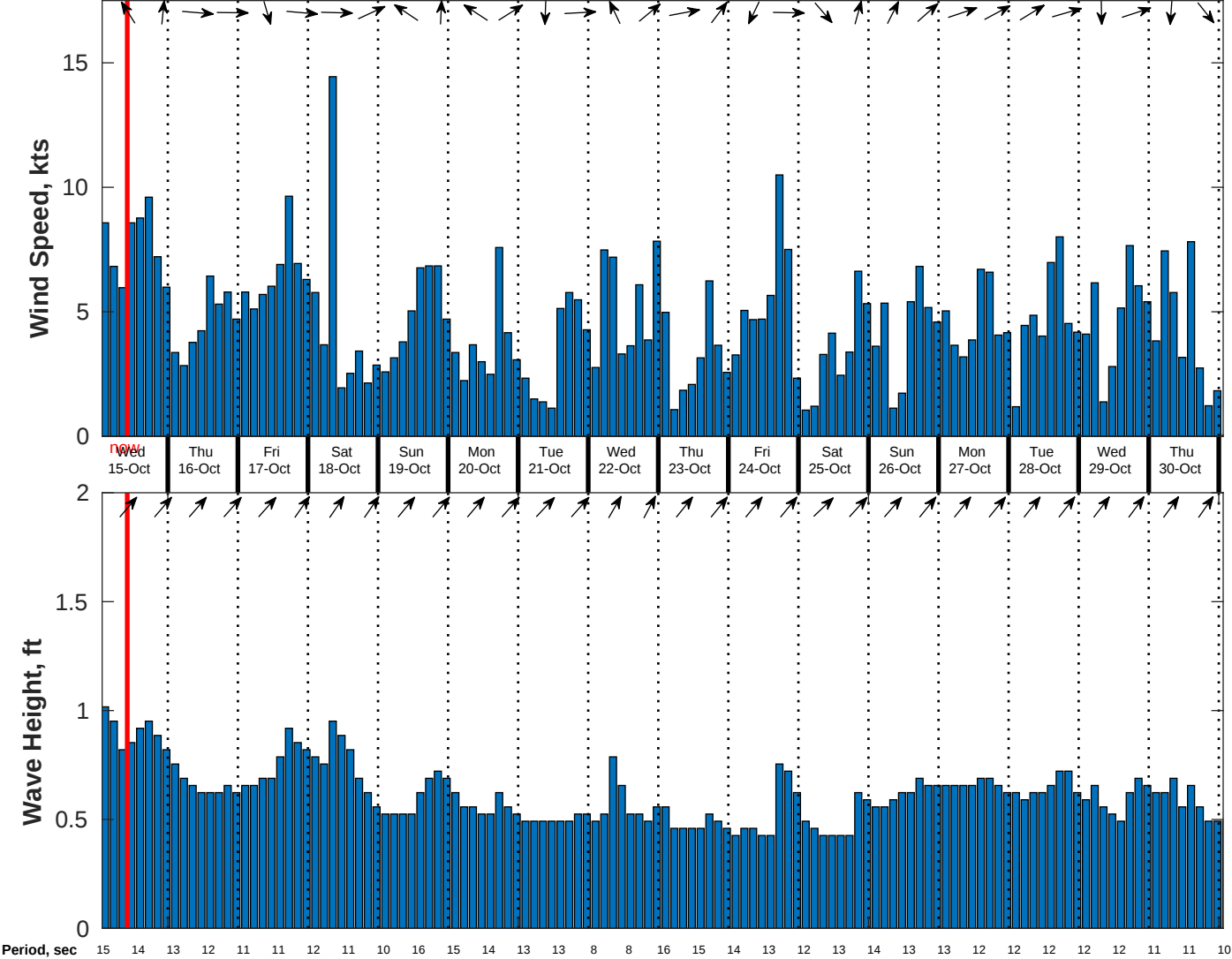
Wind & Wave Forecast for CSA (ONHYM) PPL EBS - Guinea from 14-Oct-2025 01:00:00 to 30-Oct-2025 01:00:00
