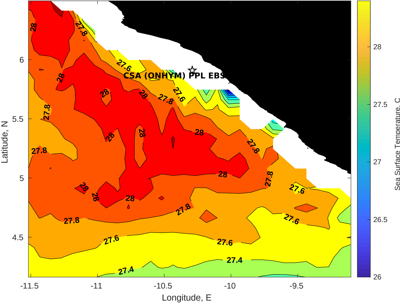
SST for CSA (ONHYM) PPL EBS - Liberia at 13-Oct-2025 00:00:00
