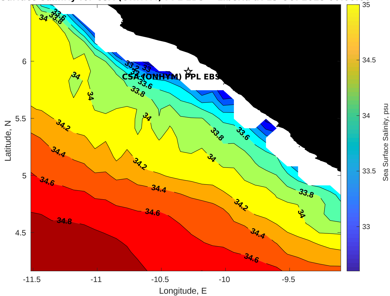
Surface Salinity for CSA (ONHYM) PPL EBS - Liberia at 13-Oct-2025 00:00:00
