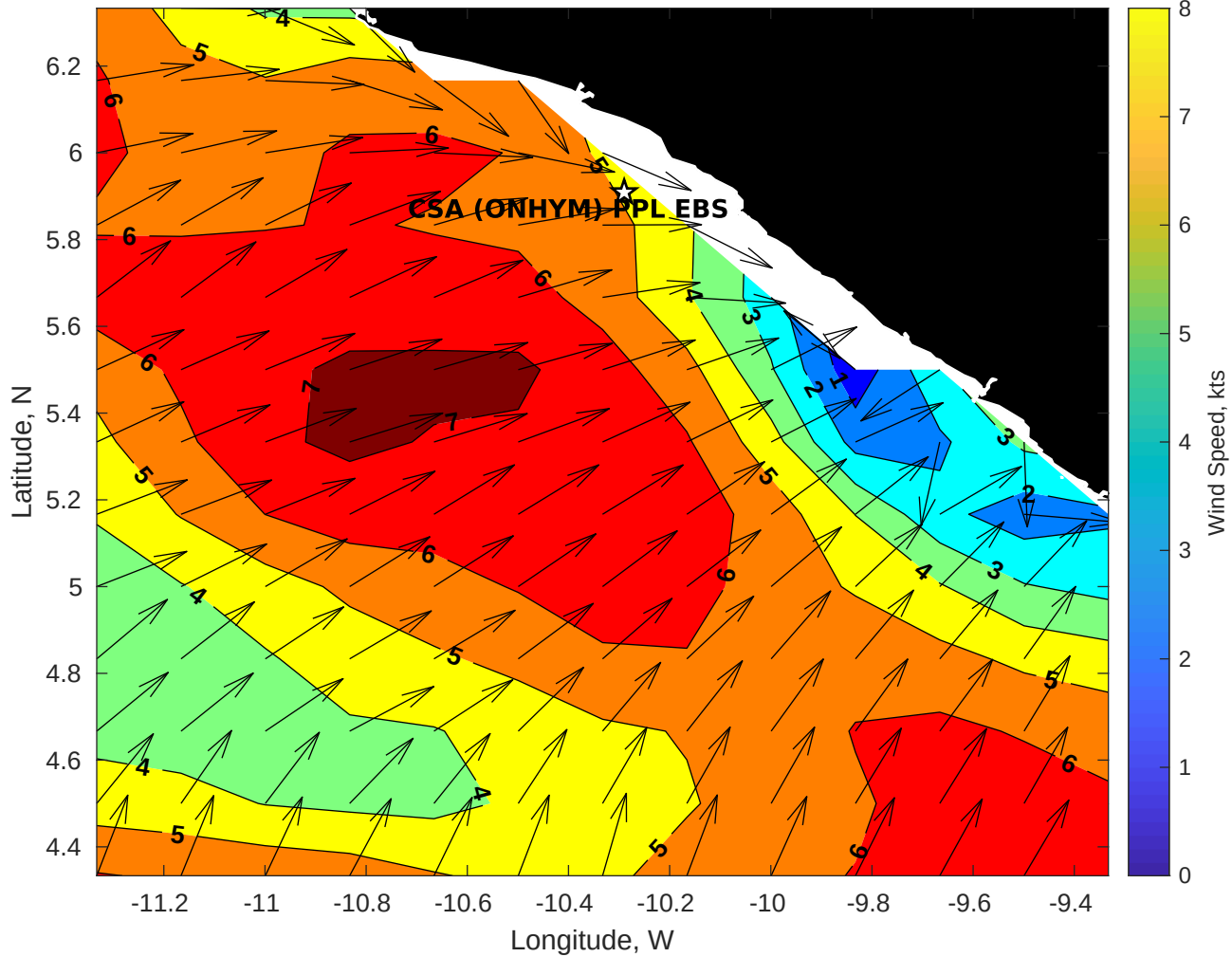
Winds (kts) for CSA (ONHYM) PPL EBS - Liberia at 14-Oct-2025 09:00:00
