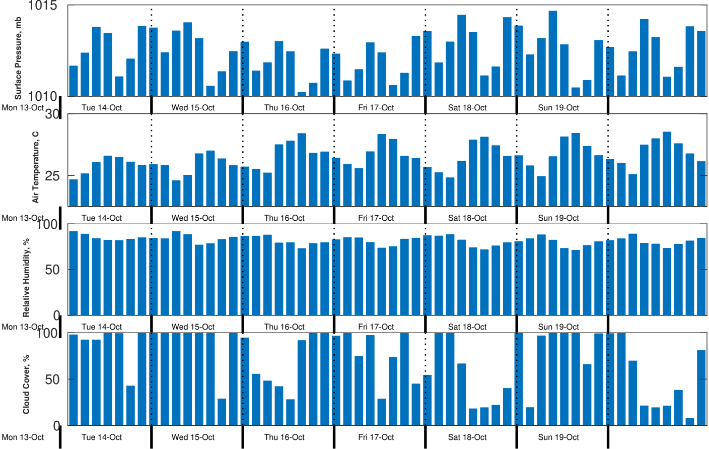
Met Forecast for CSA (ONHYM) PPL EBS - Liberia from 14-Oct-2025 00:00:00 to 21-Oct-2025 00:00:00
