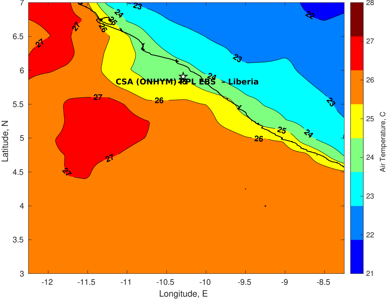
Air Temperature (C) for CSA (ONHYM) PPL EBS - Liberia at 14-Oct-2025
