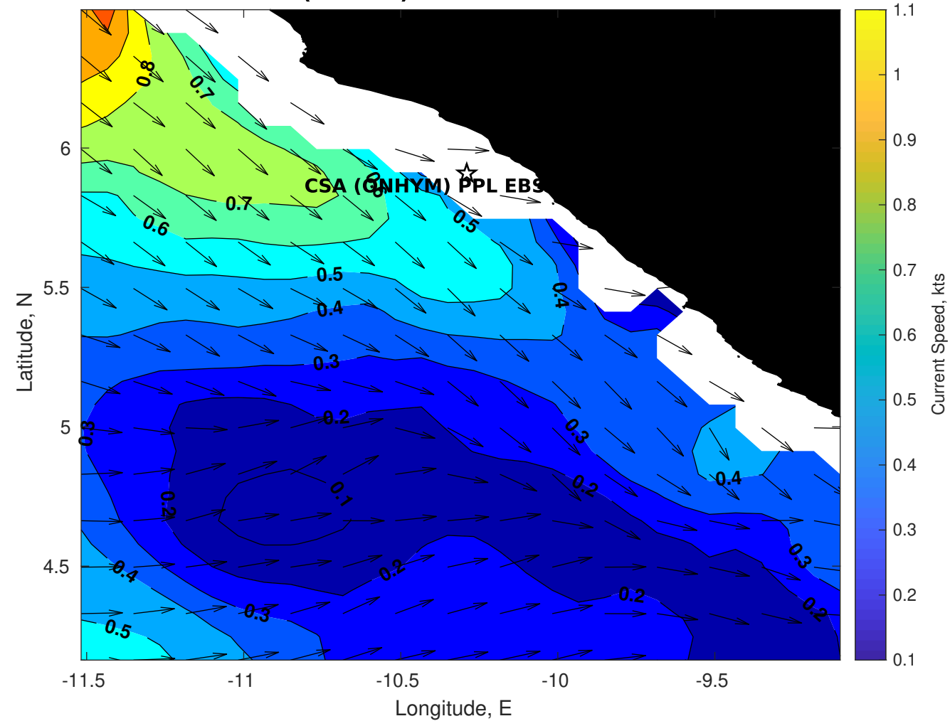
Surface Currents for CSA (ONHYM) PPL EBS - Liberia at 13-Oct-2025 00:00:00
