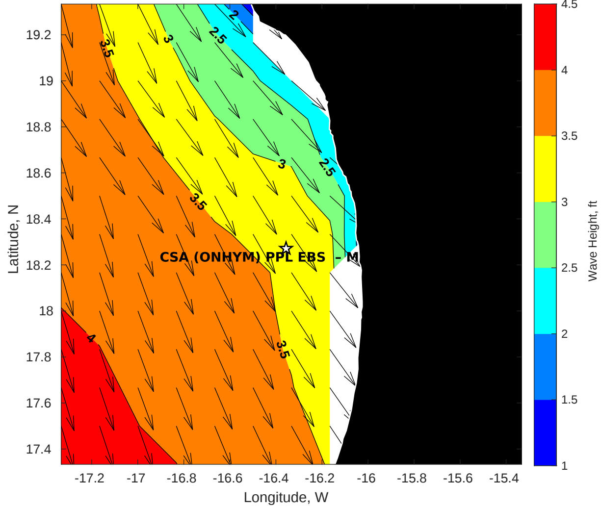
Wave Height (ft) for CSA (ONHYM) PPL EBS - Mauritania at 13-Oct-2025 21:00:00
