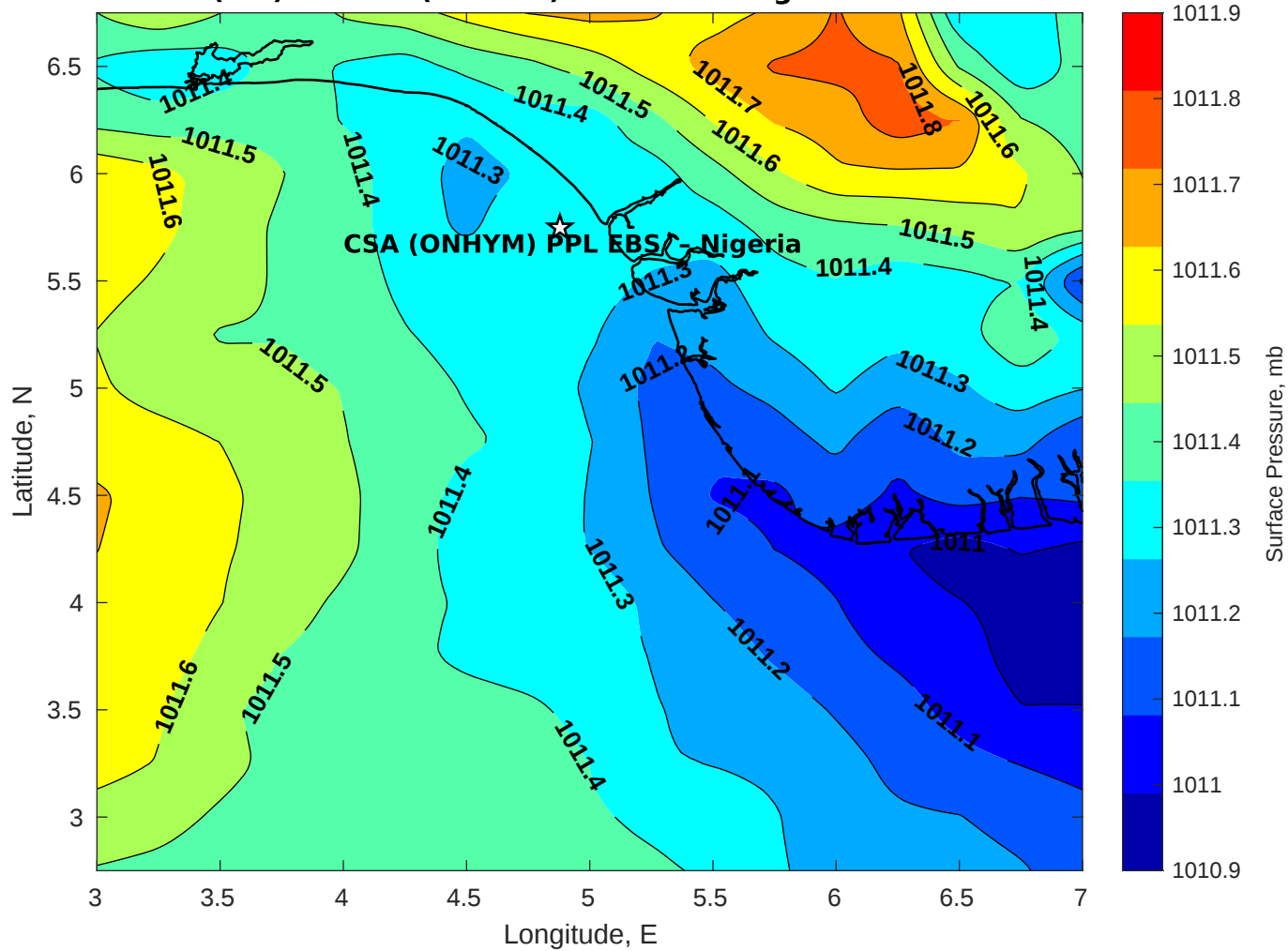
Surface Pressure (mb) for CSA (ONHYM) PPL EBS - Nigeria at 16-Oct-2025 00:00:00
