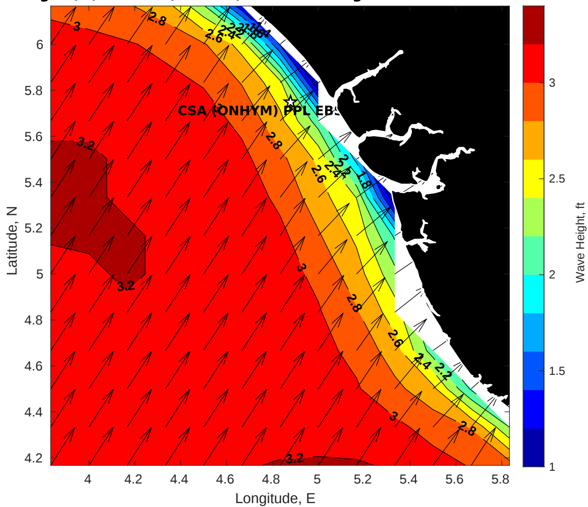
Wave Height (ft) for CSA (ONHYM) PPL EBS - Nigeria at 14-Oct-2025 09:00:00
