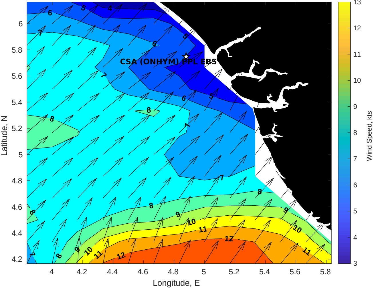
Winds (kts) for CSA (ONHYM) PPL EBS - Nigeria at 14-Oct-2025 09:00:00
