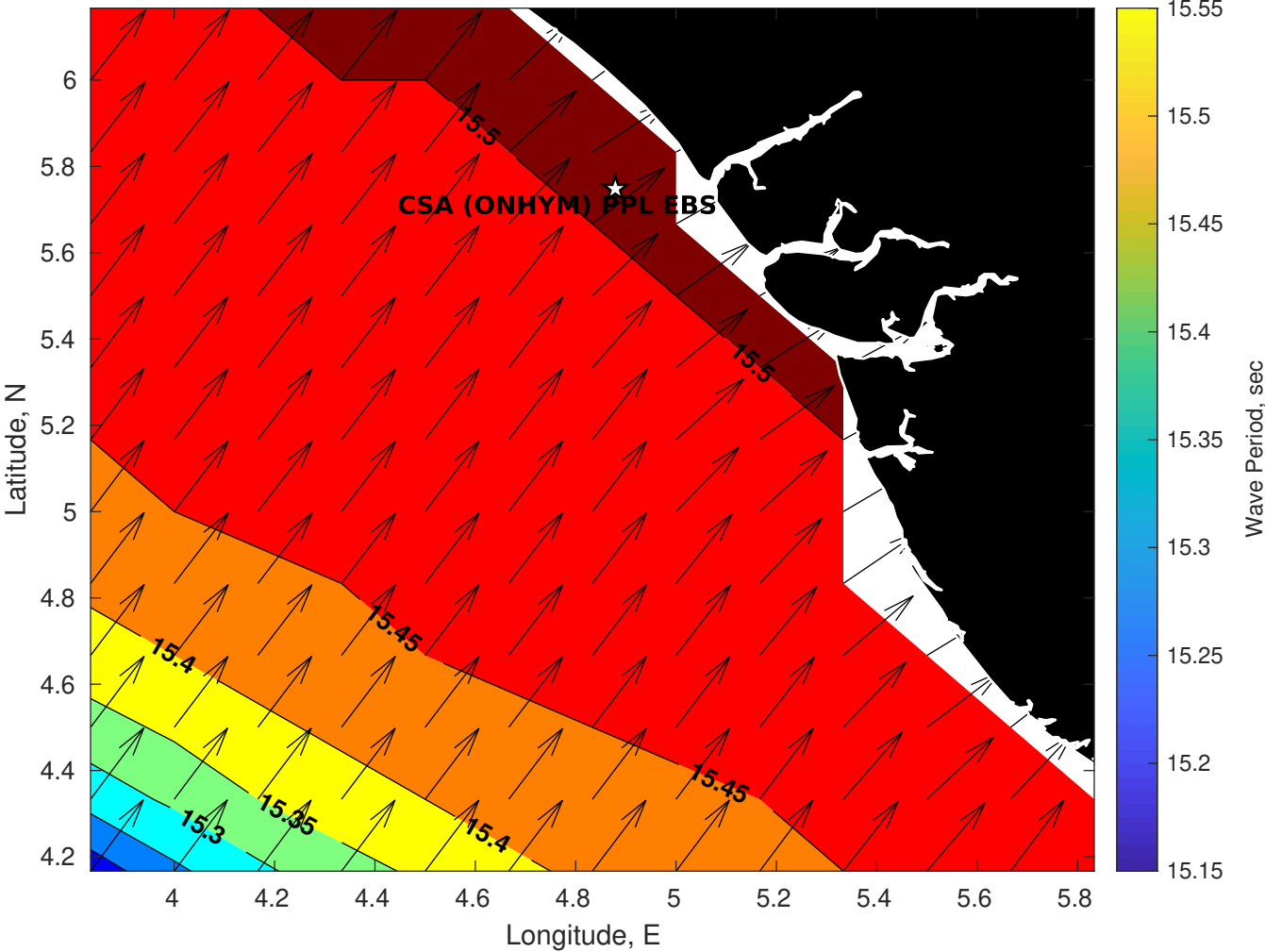
Wave Period (sec) for CSA (ONHYM) PPL EBS - Nigeria at 14-Oct-2025 09:00:00
