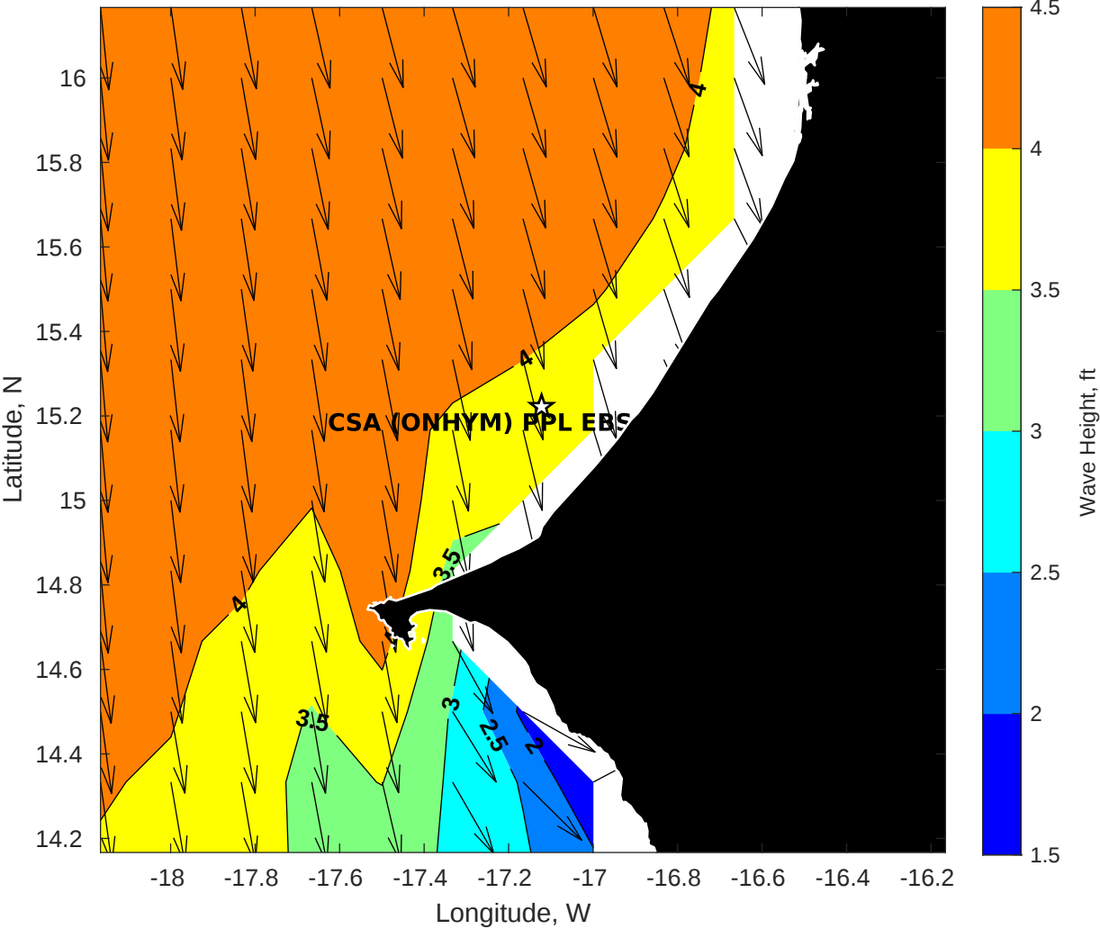
Wave Height (ft) for CSA (ONHYM) PPL EBS - Senegal at 13-Oct-2025 21:00:00
