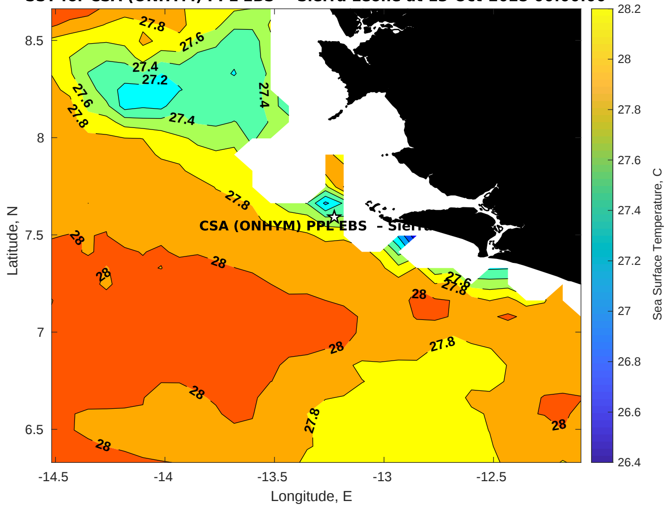
SST for CSA (ONHYM) PPL EBS - Sierra Leone at 13-Oct-2025 00:00:00
