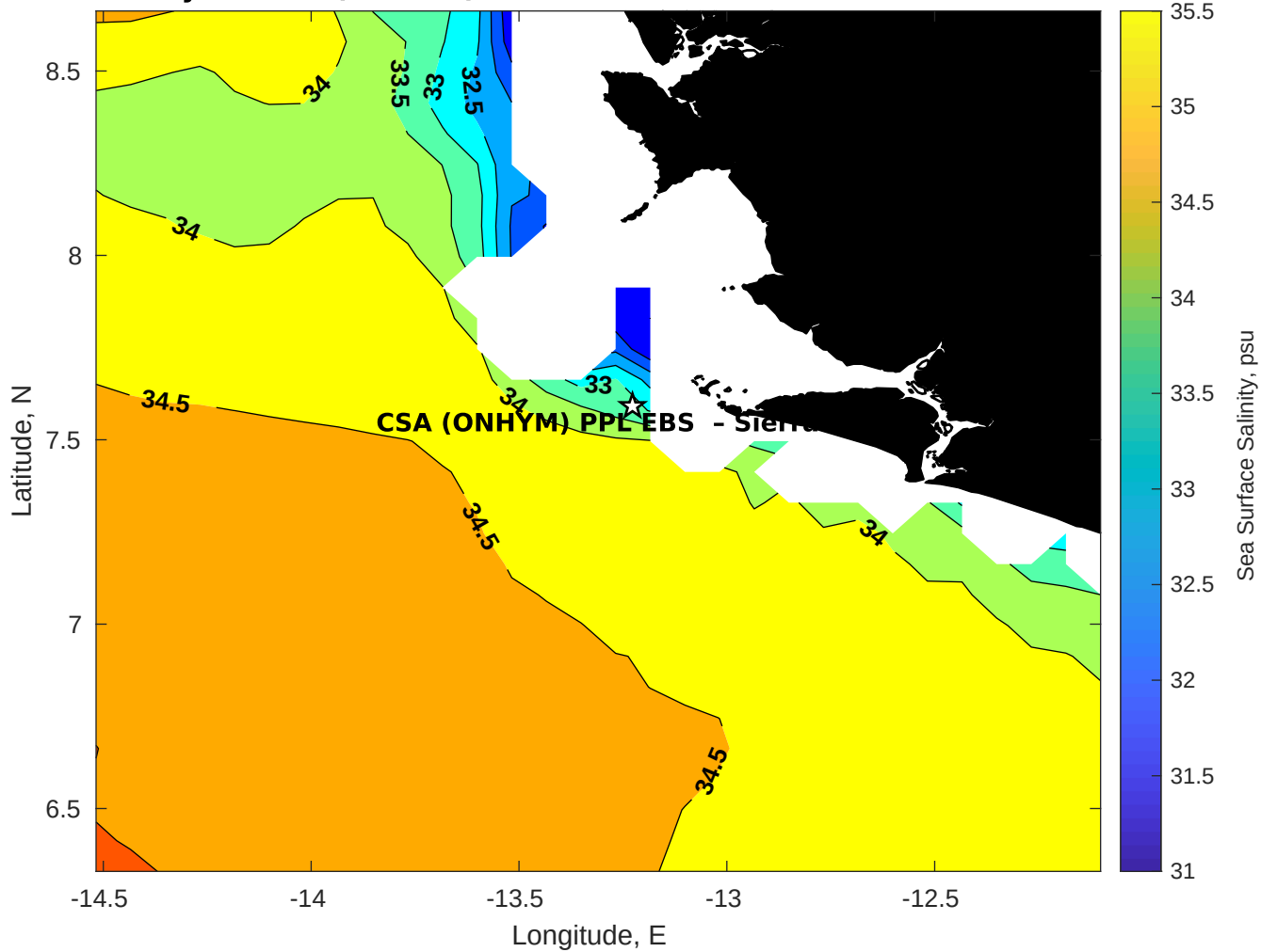
Surface Salinity for CSA (ONHYM) PPL EBS - Sierra Leone at 13-Oct-2025 00:00:00
