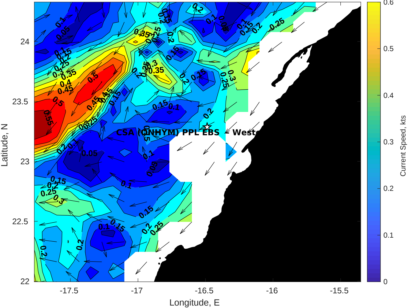
Surface Currents for CSA (ONHYM) PPL EBS - Western Sahara at 13-Oct-2025 00:00:00
