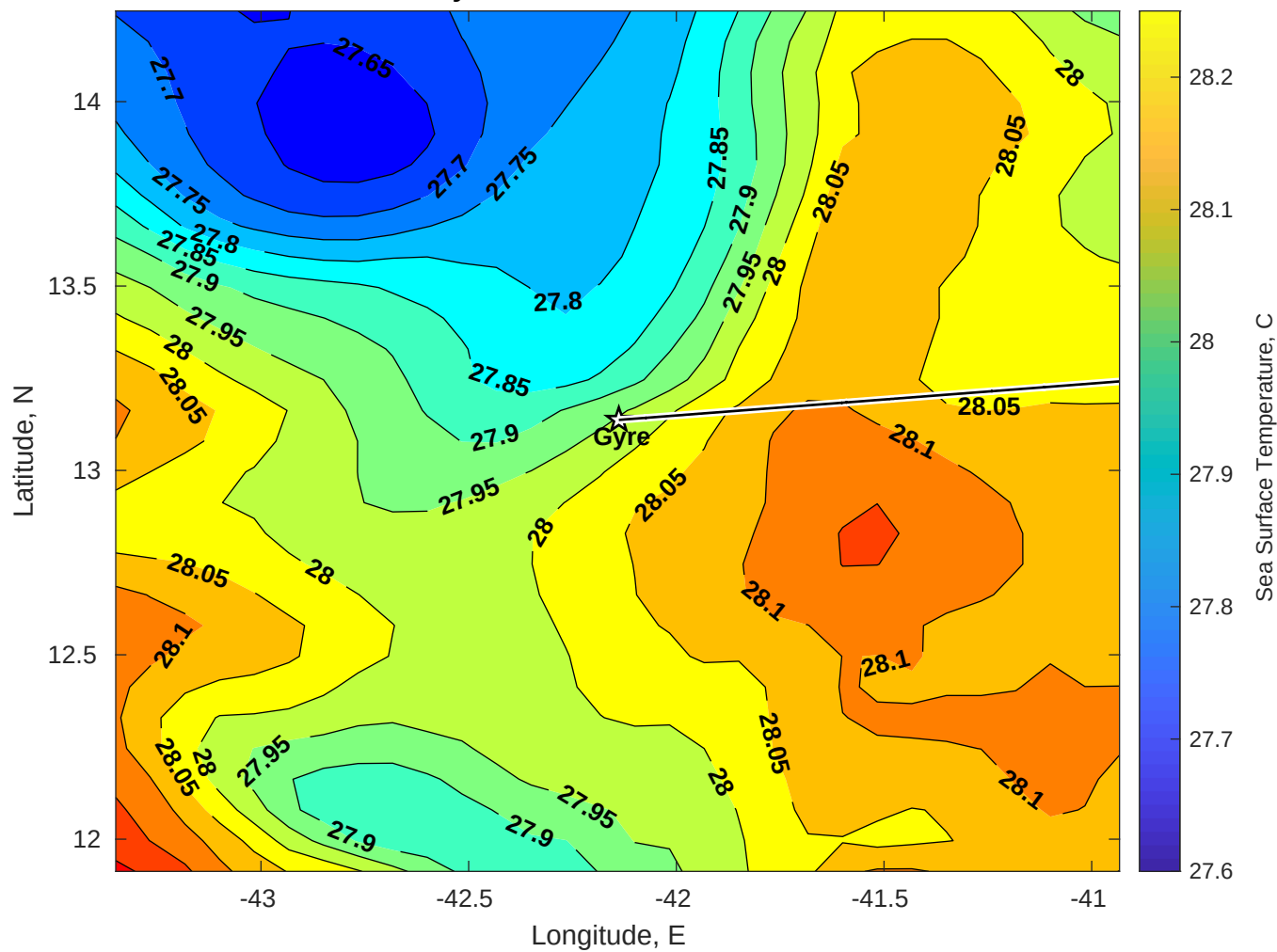
SST for Gyre at 13-Oct-2025 00:00:00
