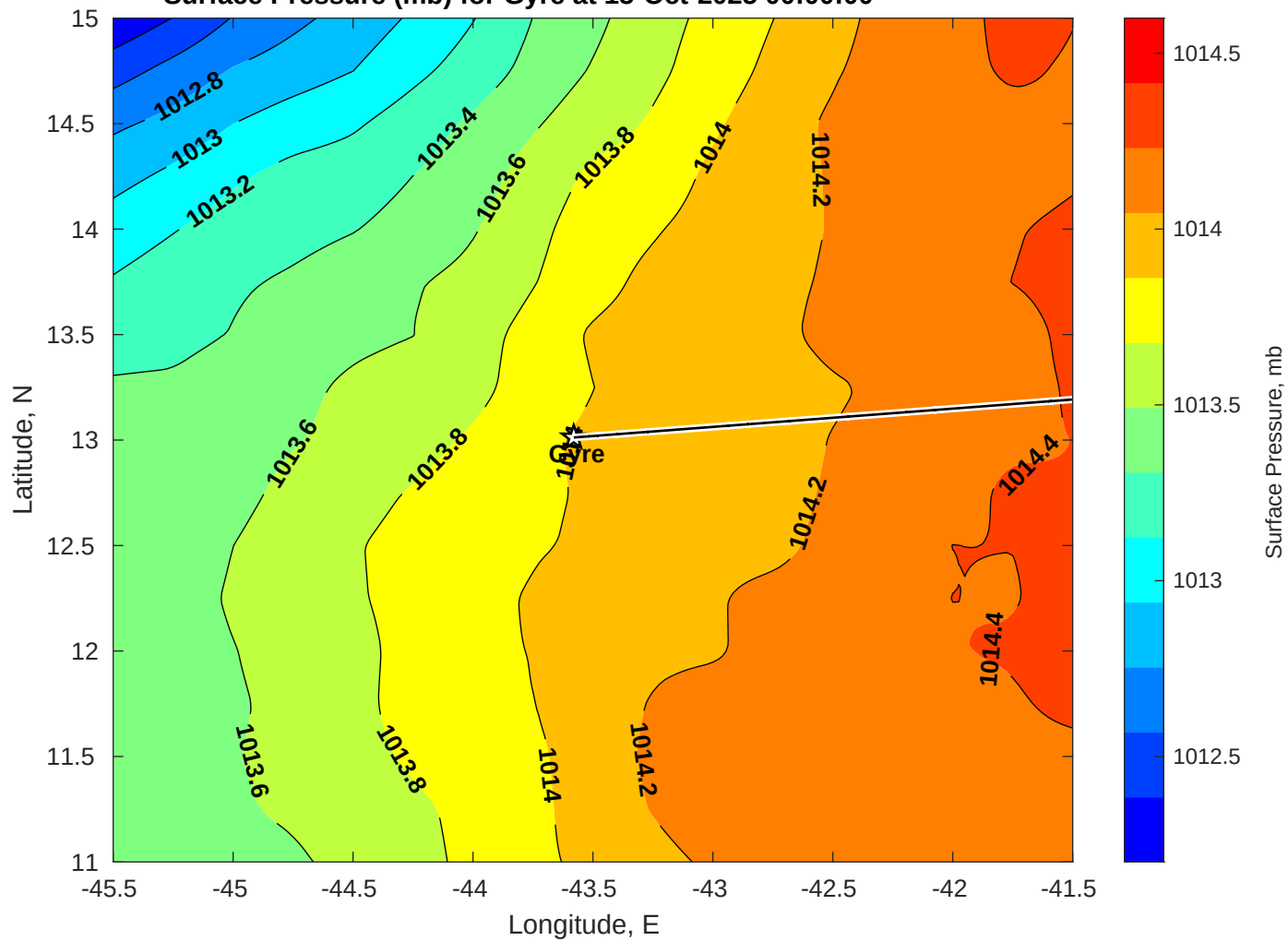
Surface Pressure (mb) for Gyre at 15-Oct-2025 00:00:00
