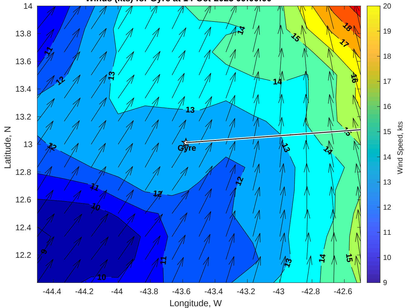
Winds (kts) for Gyre at 14-Oct-2025 09:00:00
