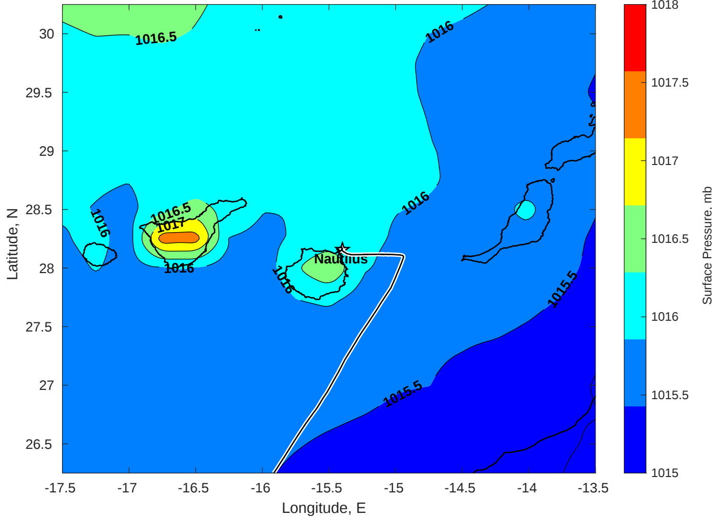
Surface Pressure (mb) for Nautilus at 14-Oct-2025 00:00:00
