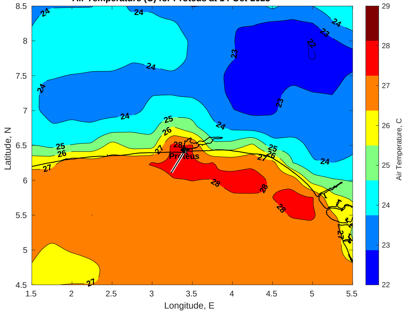
Air Temperature (C) for Proteus at 14-Oct-2025
